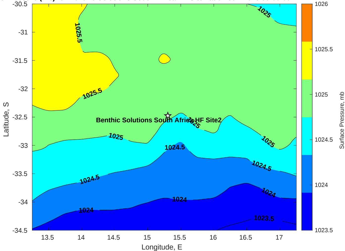
Surface Pressure (mb) for Benthic Solutions South Africa HF Site2 at 01-Jun-2025 00:00:00
