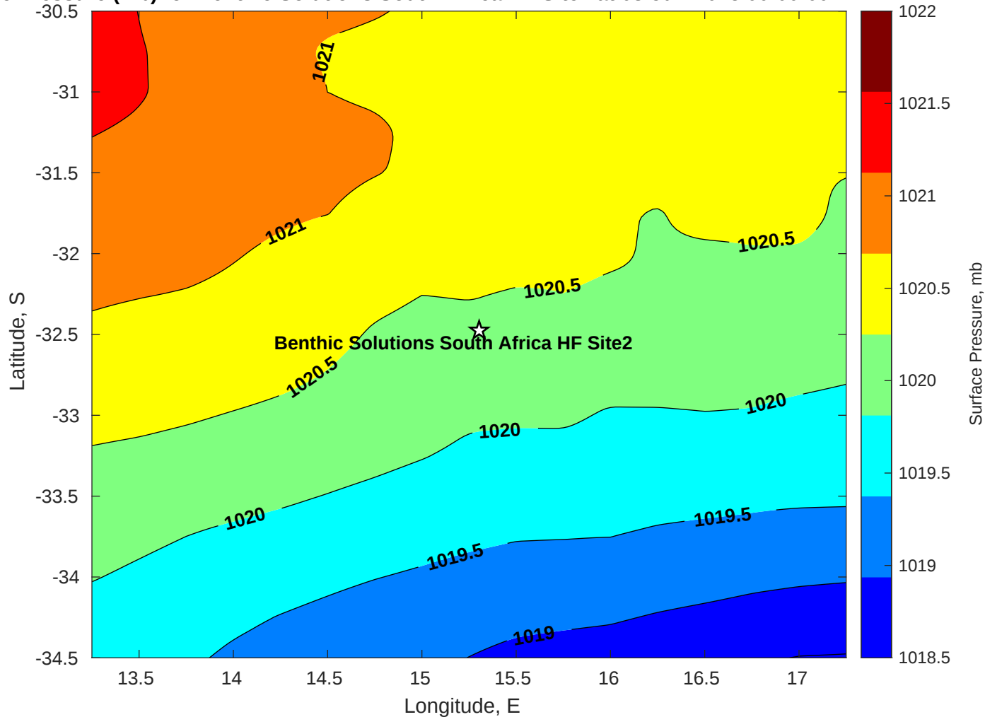
Surface Pressure (mb) for Benthic Solutions South Africa HF Site2 at 03-Jun-2025 00:00:00
