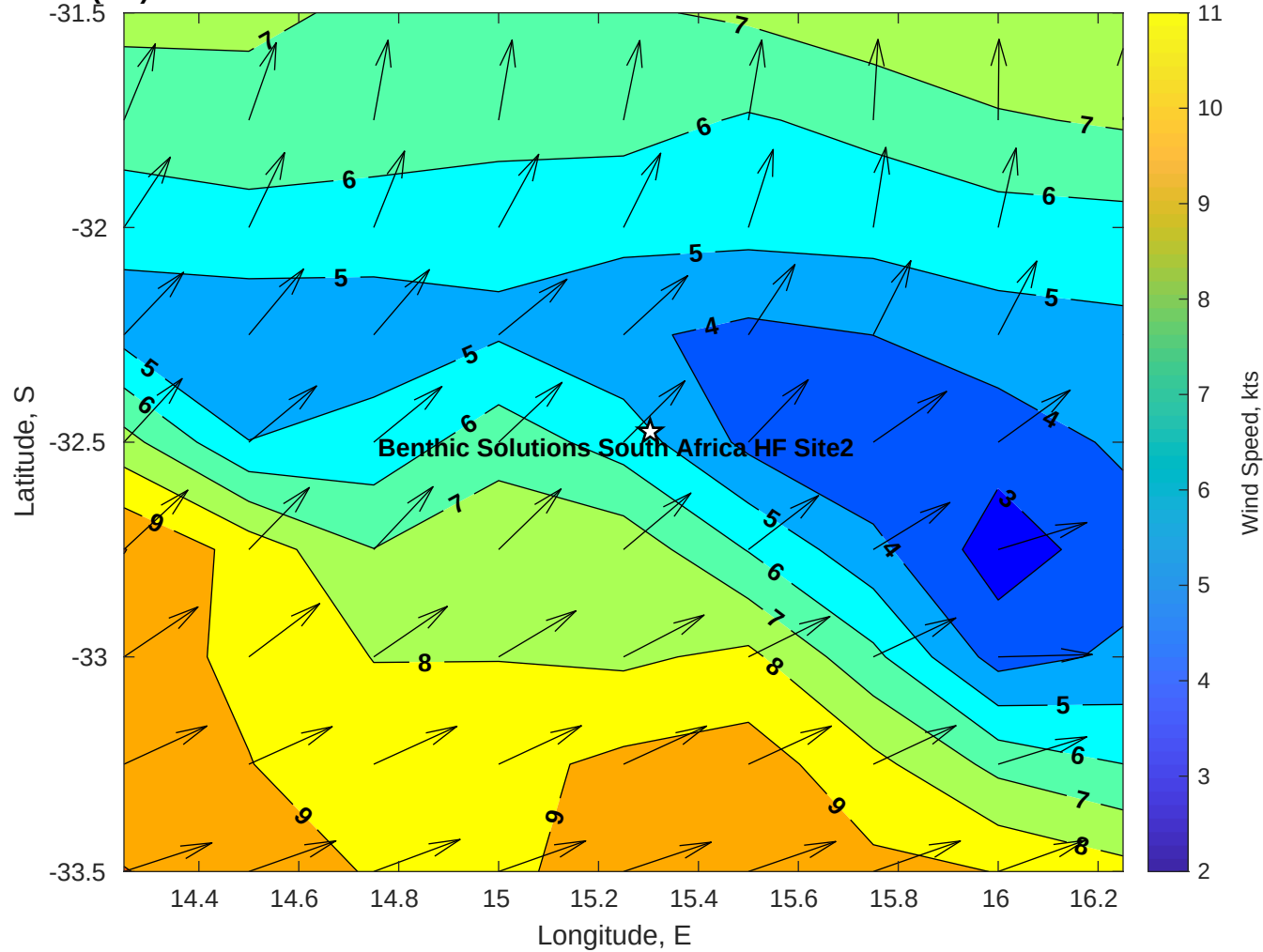
Winds (kts) for Benthic Solutions South Africa HF Site2 at 01-Jun-2025 09:00:00
