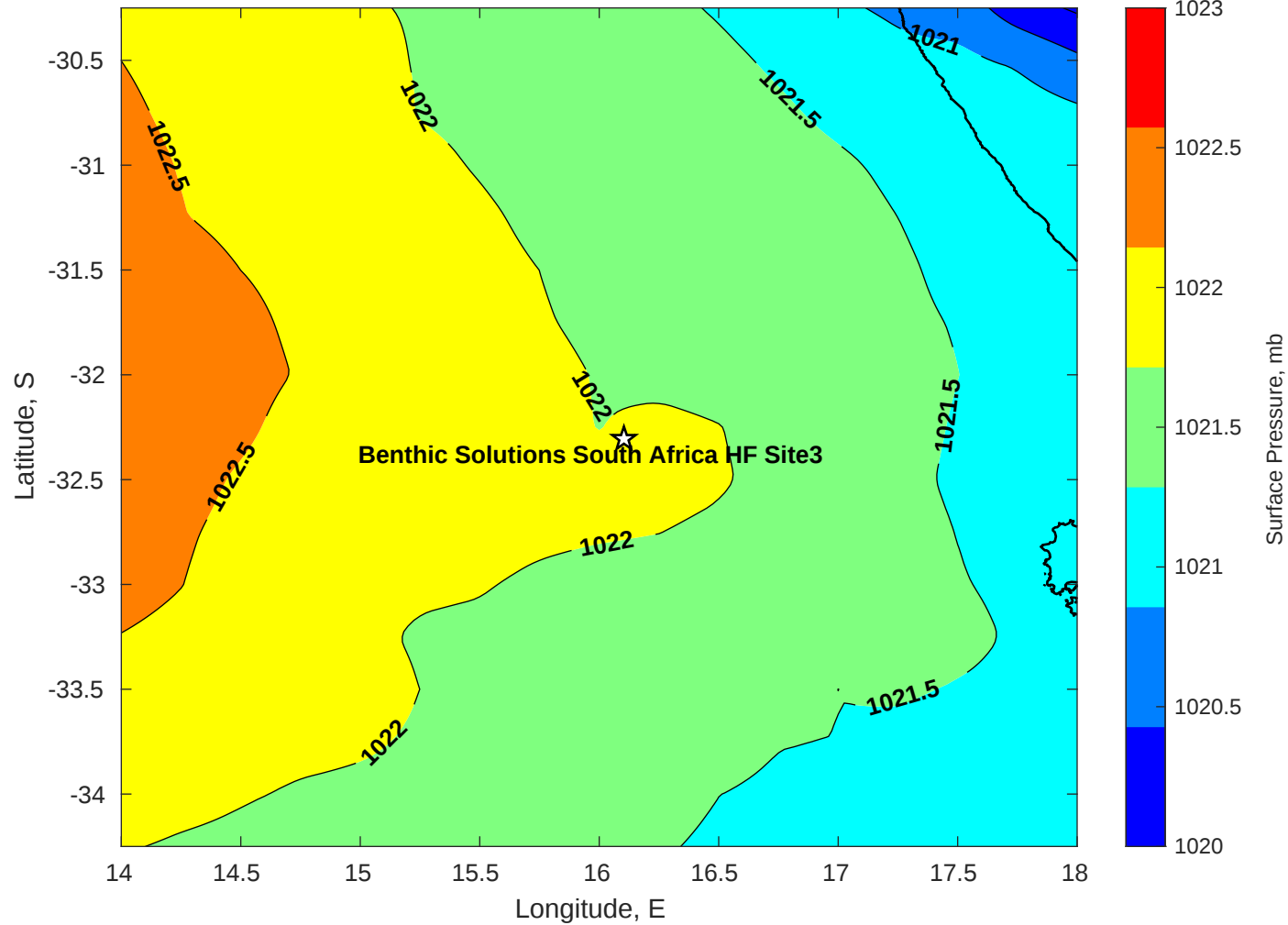
Surface Pressure (mb) for Benthic Solutions South Africa HF Site3 at 02-Jun-2025 00:00:00
