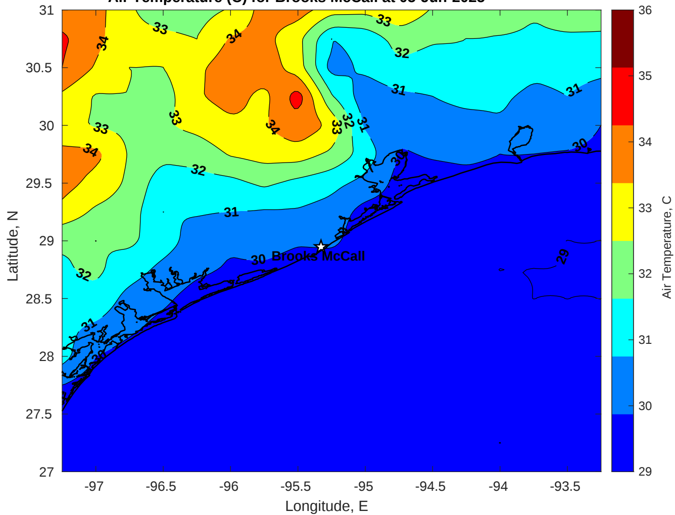
Air Temperature (C) for Brooks McCall at 05-Jun-2025
