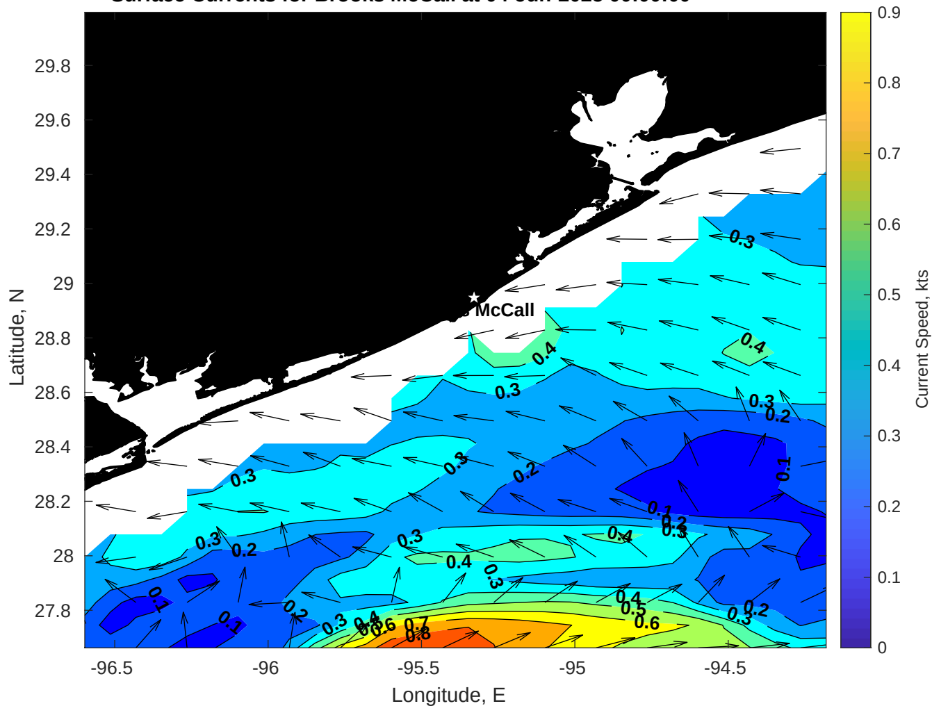
Surface Currents for Brooks McCall at 04-Jun-2025 00:00:00
