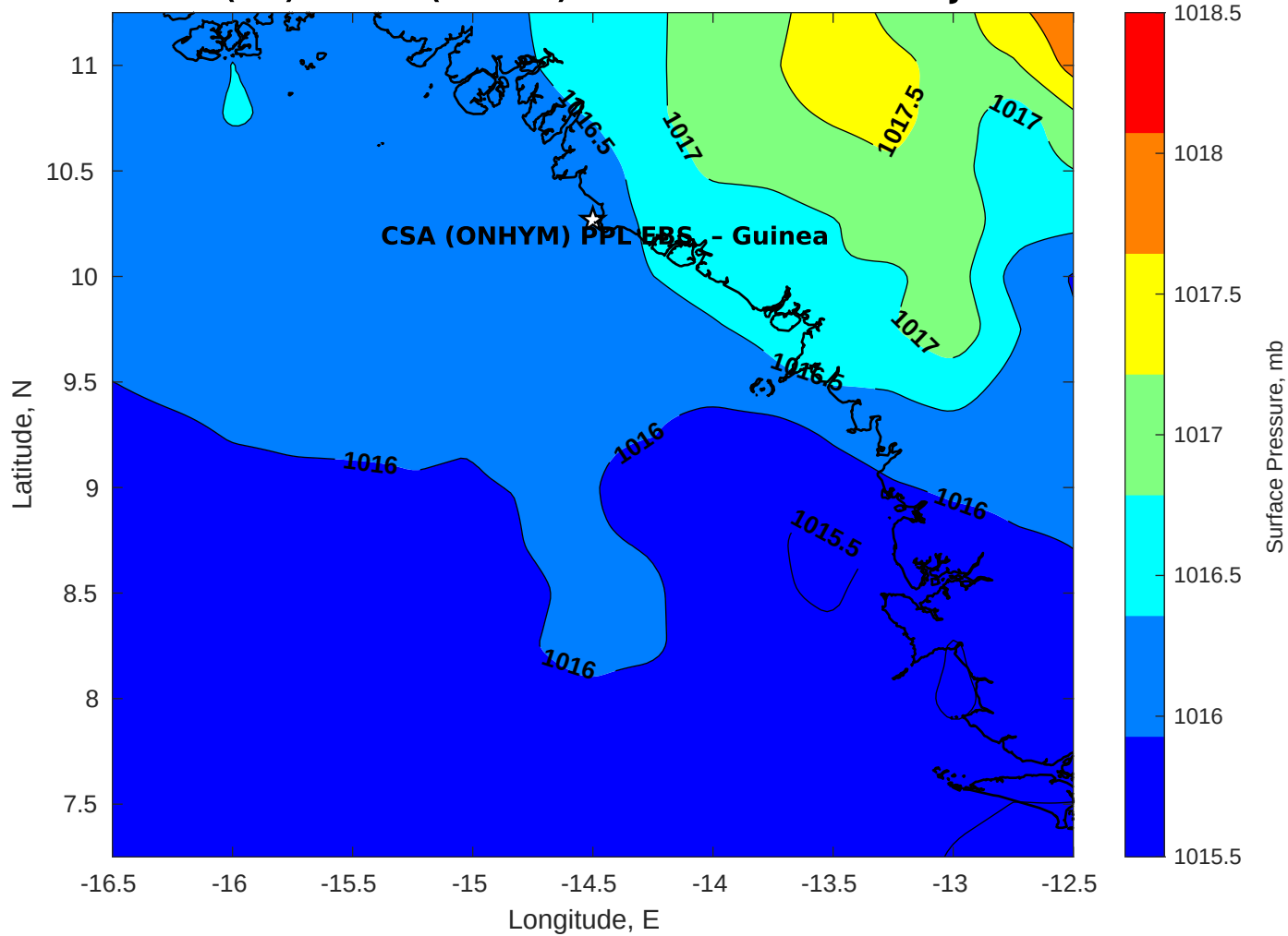
Surface Pressure (mb) for CSA (ONHYM) PPL EBS - Guinea at 01-Jun-2025 00:00:00
