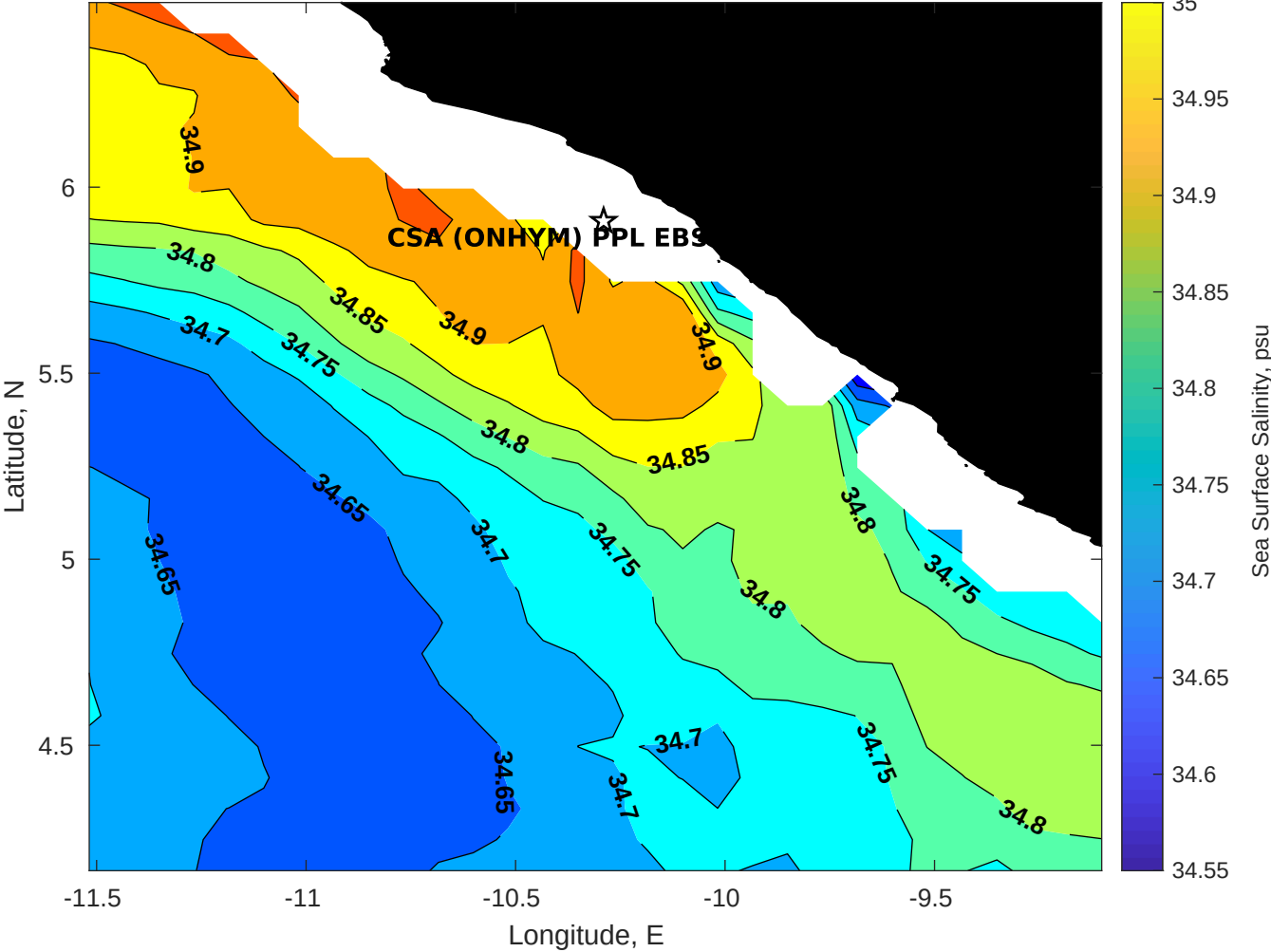
Surface Salinity for CSA (ONHYM) PPL EBS - Liberia at 26-May-2025 00:00:00
