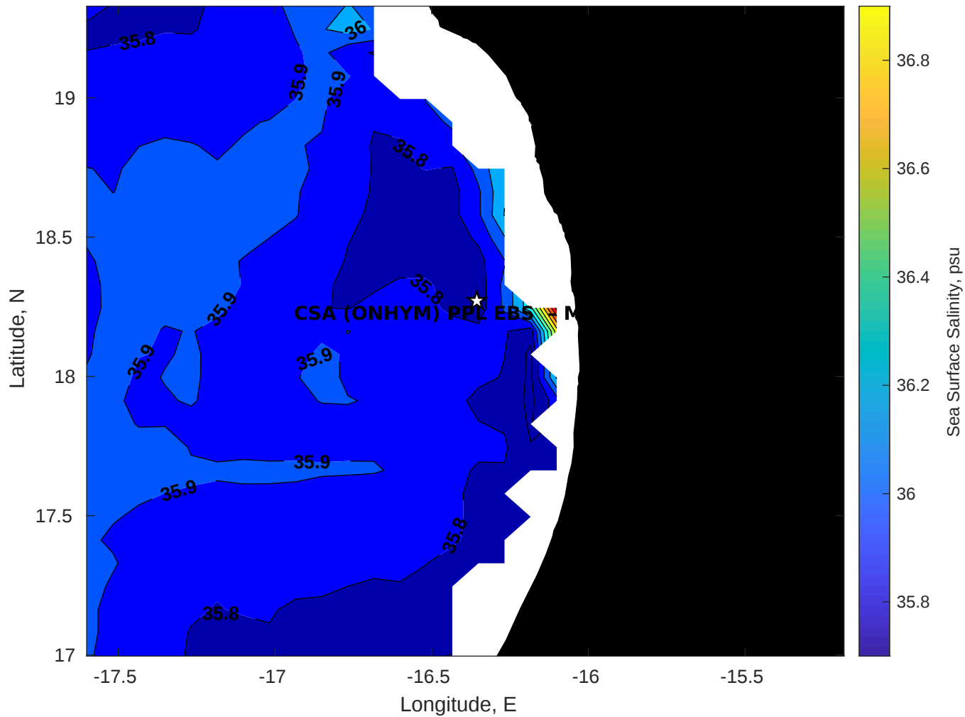
Surface Salinity for CSA (ONHYM) PPL EBS - Mauritania at 26-May-2025 00:00:00
