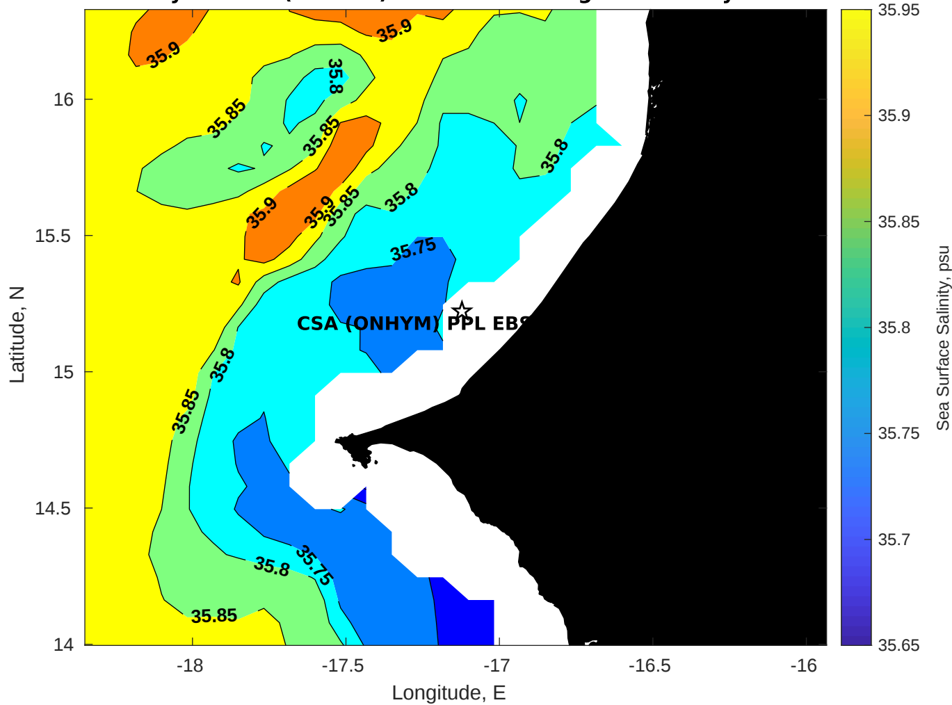
Surface Salinity for CSA (ONHYM) PPL EBS - Senegal at 26-May-2025 00:00:00
