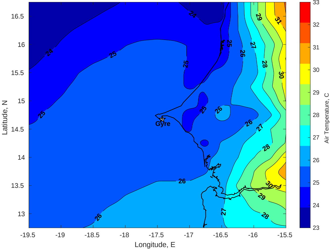
Air Temperature (C) for Gyre at 05-Jun-2025
