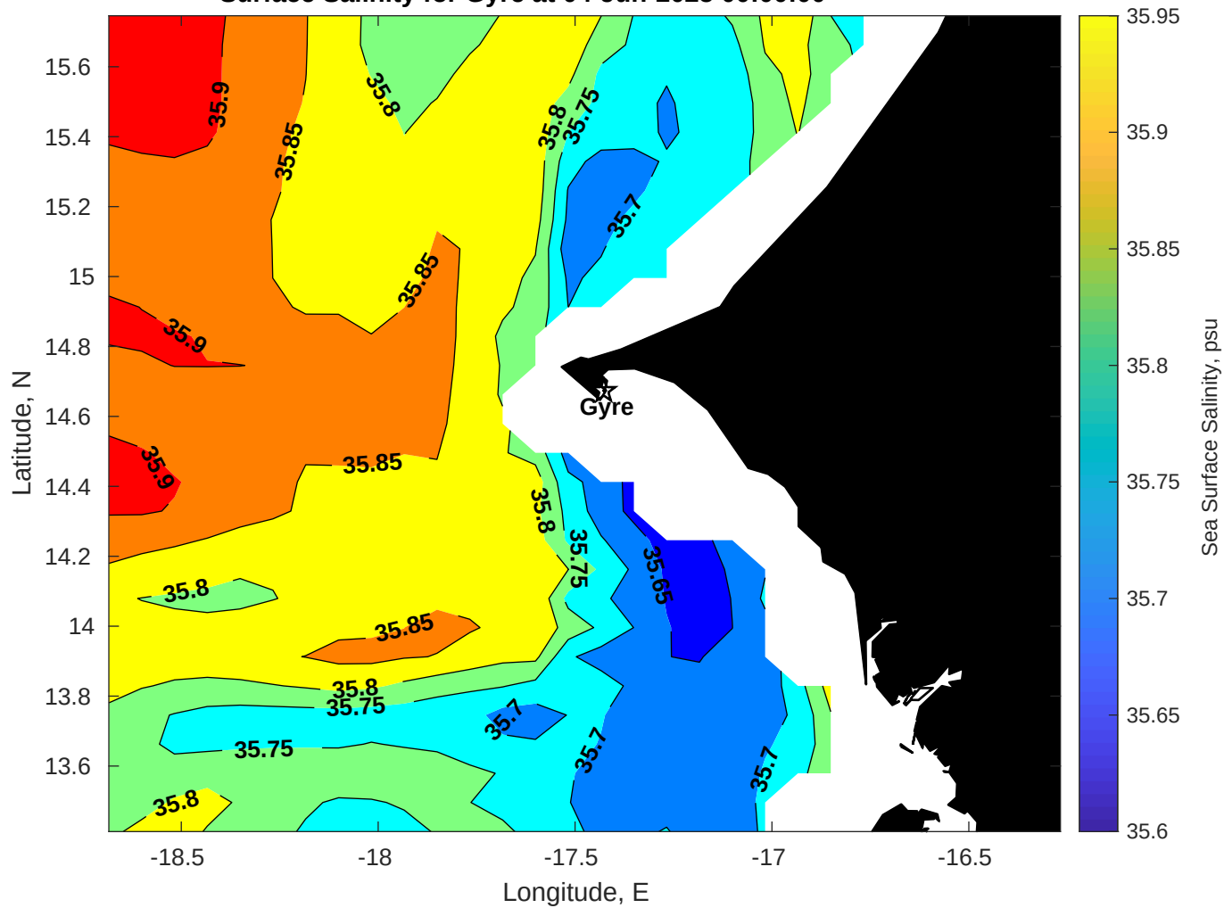
Surface Salinity for Gyre at 04-Jun-2025 00:00:00
