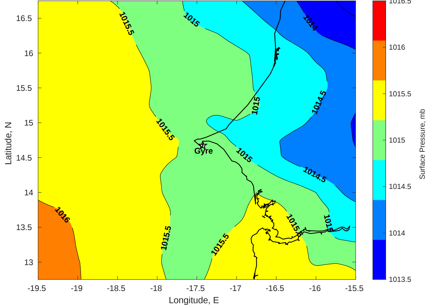
Surface Pressure (mb) for Gyre at 06-Jun-2025 00:00:00
