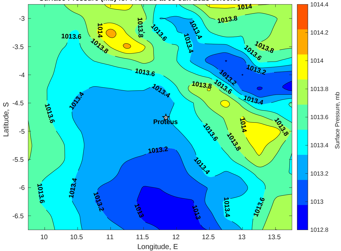
Surface Pressure (mb) for Proteus at 03-Jun-2025 00:00:00
