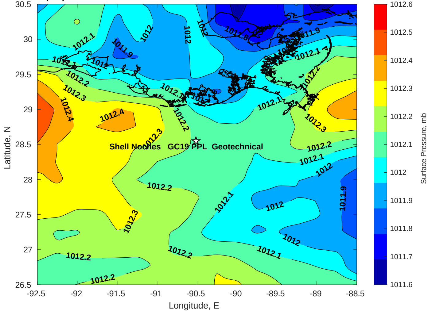
Surface Pressure (mb) for Shell Noches GC19 PPL Geotechnical at 01-Jun-2025 00:00:00
