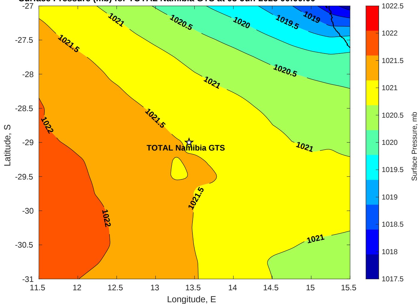
Surface Pressure (mb) for TOTAL Namibia GTS at 03-Jun-2025 00:00:00
