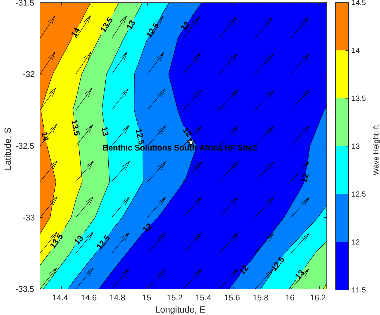
Wave Height (ft) for Benthic Solutions South Africa HF Site2 at 01-Jun-2025 09:00:00
