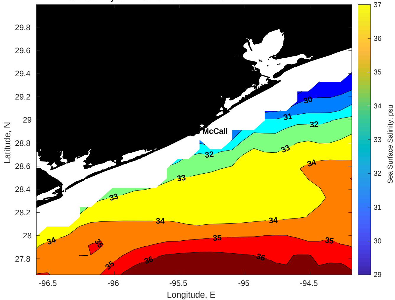
Surface Salinity for Brooks McCall at 05-Jun-2025 00:00:00
