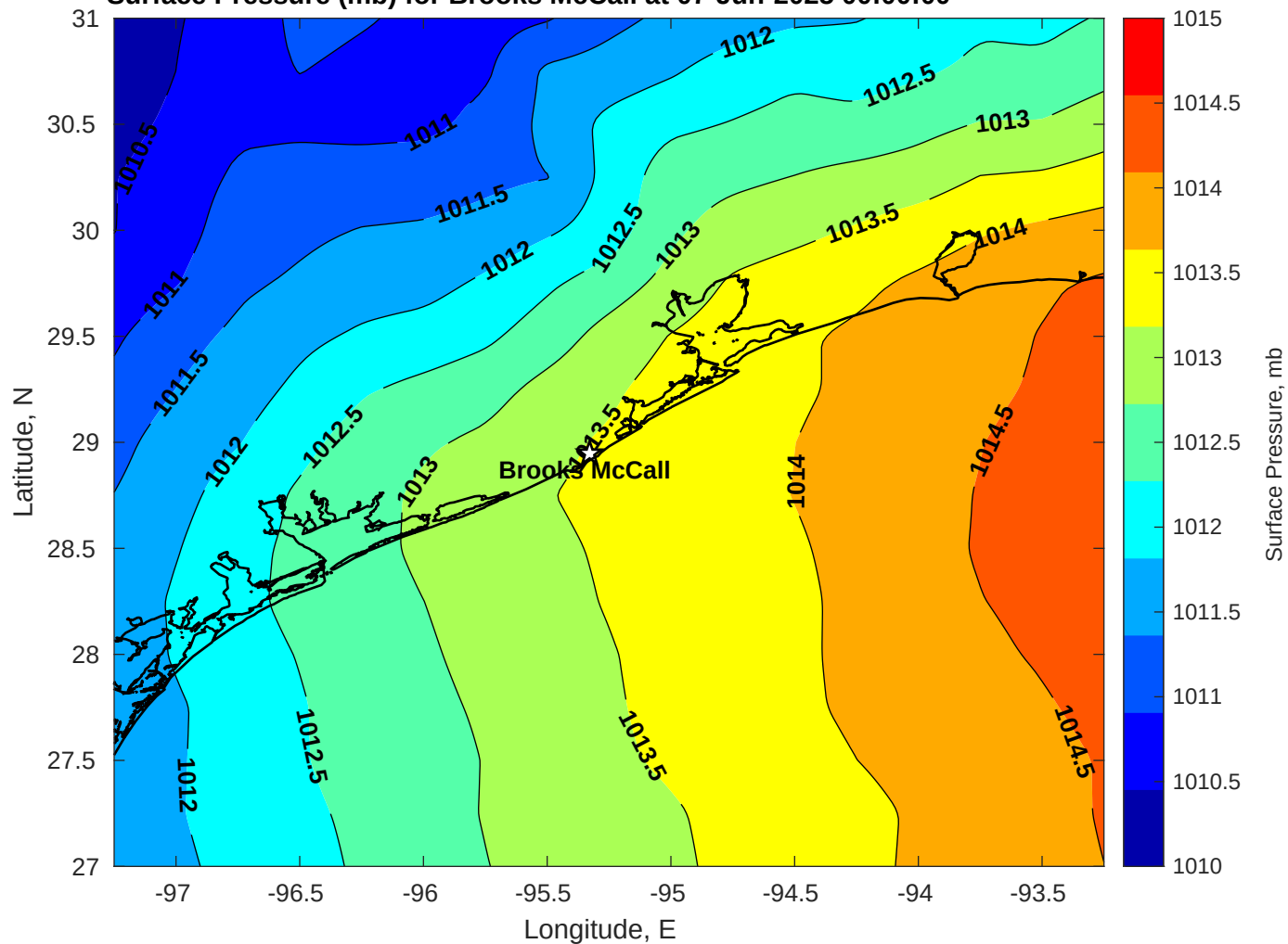
Surface Pressure (mb) for Brooks McCall at 07-Jun-2025 00:00:00
