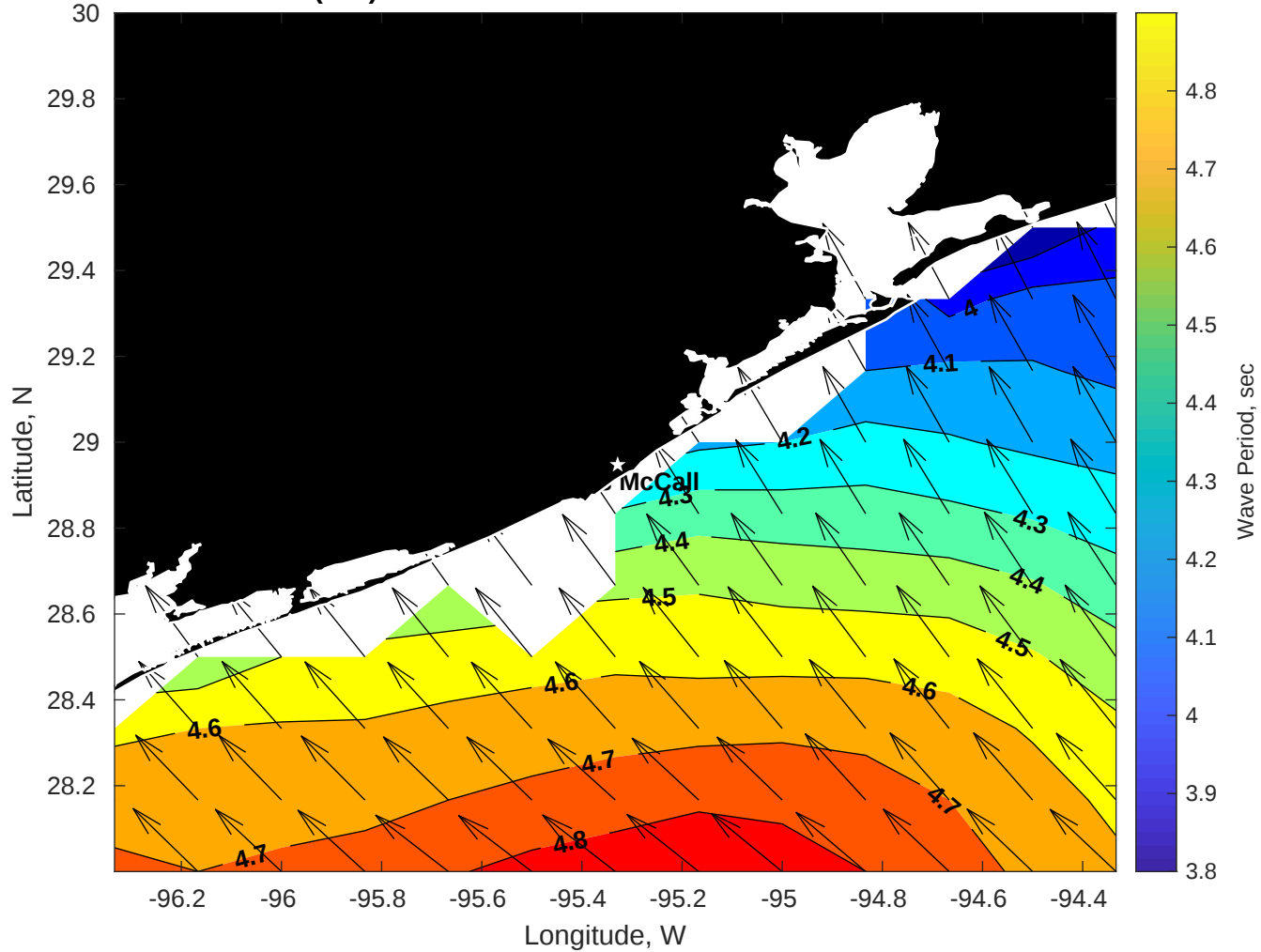
Wave Period (sec) for Brooks McCall at 06-Jun-2025 09:00:00
