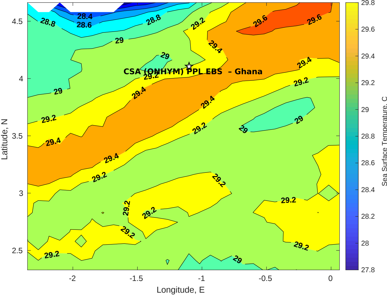
SST for CSA (ONHYM) PPL EBS - Ghana at 26-May-2025 00:00:00
