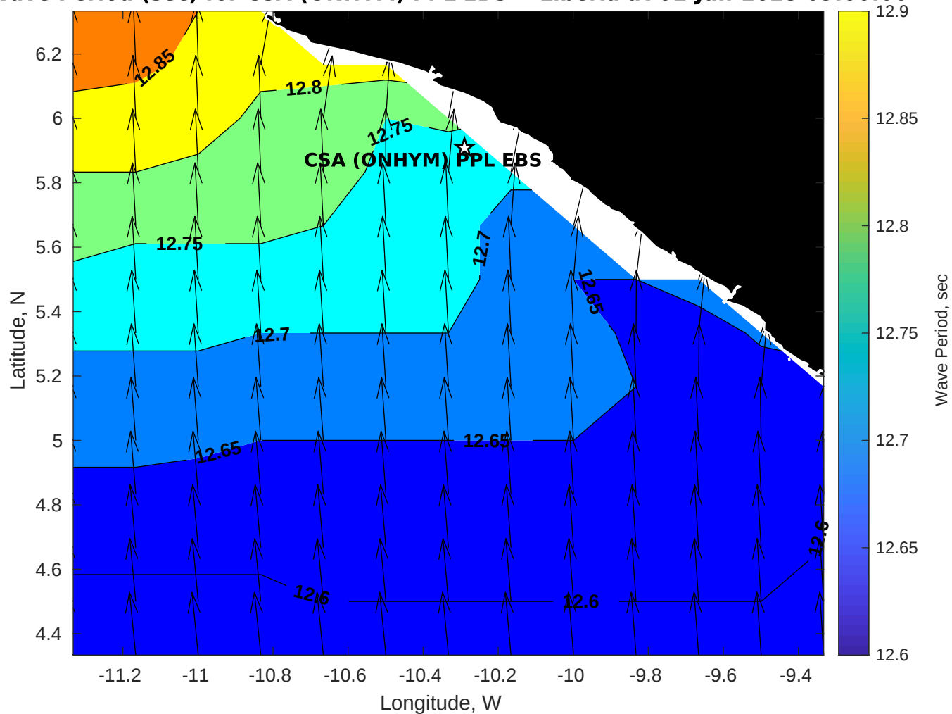
Wave Period (sec) for CSA (ONHYM) PPL EBS - Liberia at 01-Jun-2025 09:00:00
