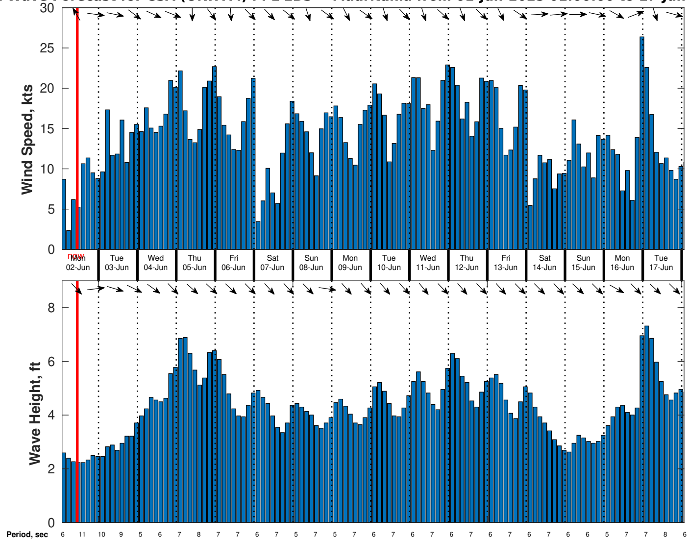
Wind & Wave Forecast for CSA (ONHYM) PPL EBS - Mauritania from 01-Jun-2025 01:00:00 to 17-Jun-2025 01:00:00
