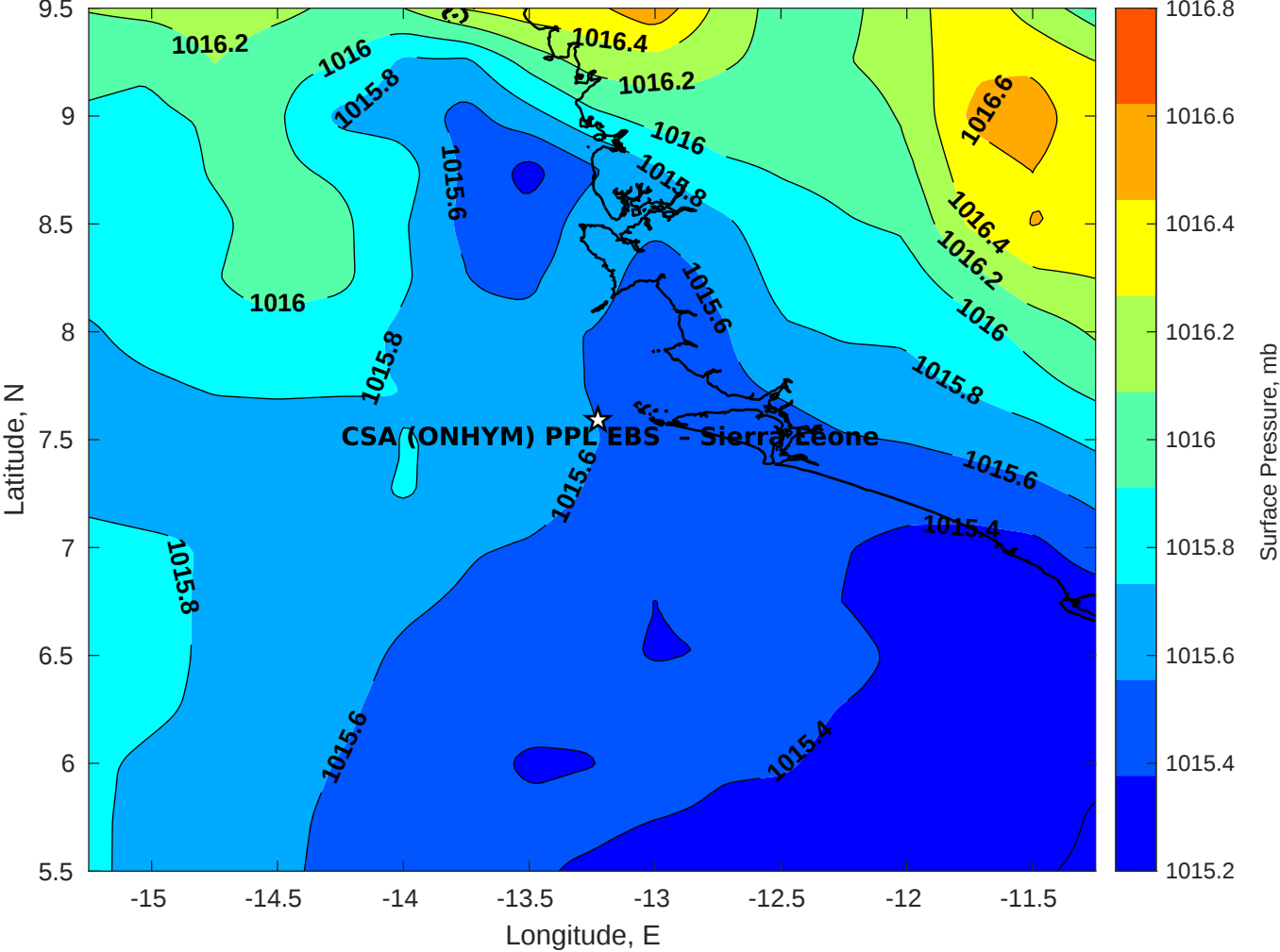
Surface Pressure (mb) for CSA (ONHYM) PPL EBS - Sierra Leone at 01-Jun-2025 00:00:00
