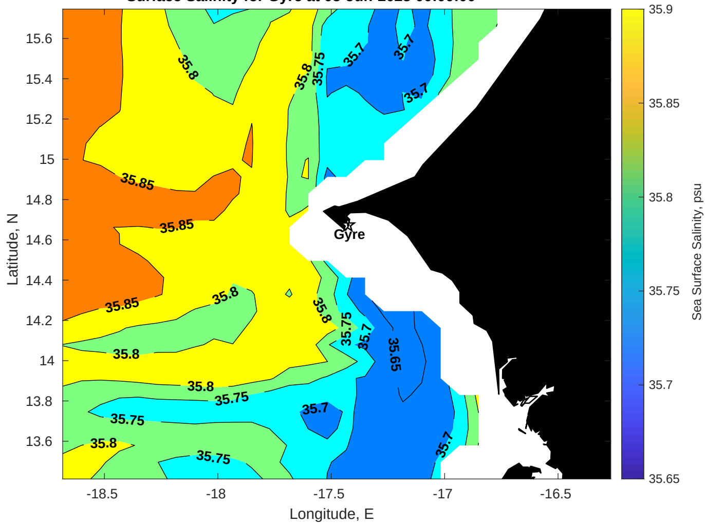
Surface Salinity for Gyre at 05-Jun-2025 00:00:00
