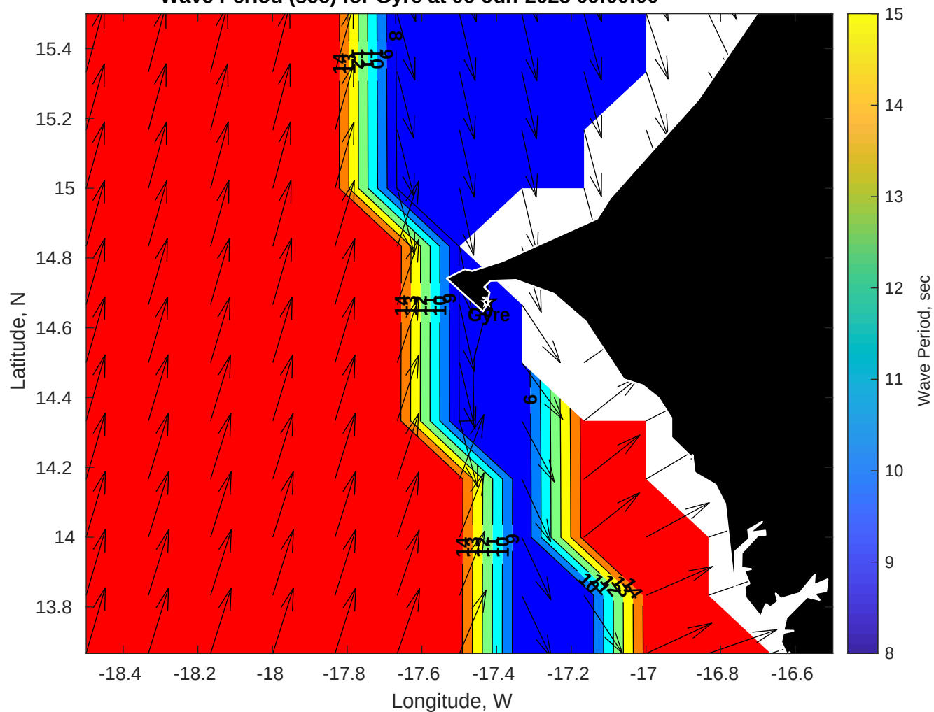
Wave Period (sec) for Gyre at 06-Jun-2025 09:00:00
