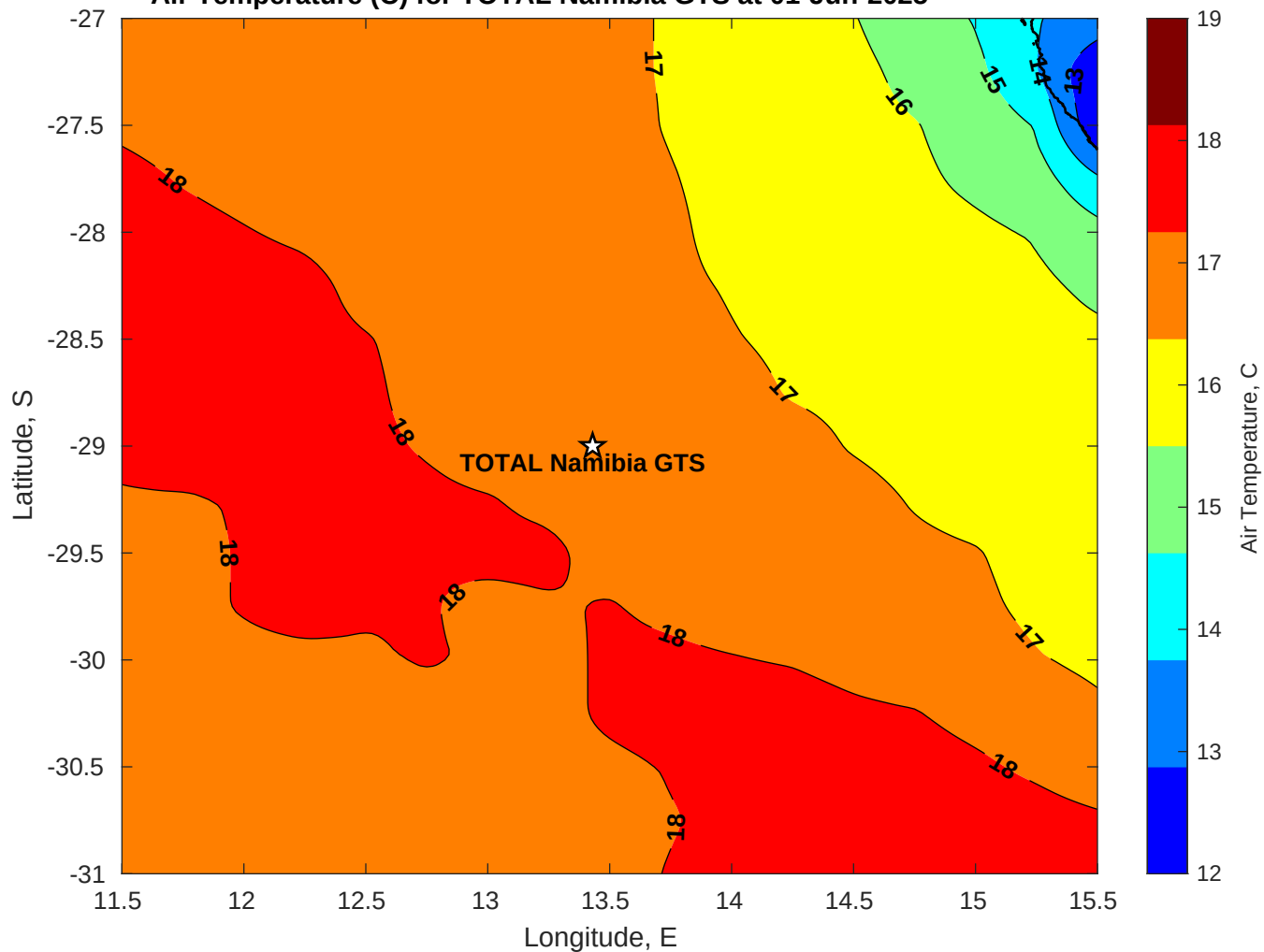
Air Temperature (C) for TOTAL Namibia GTS at 01-Jun-2025
