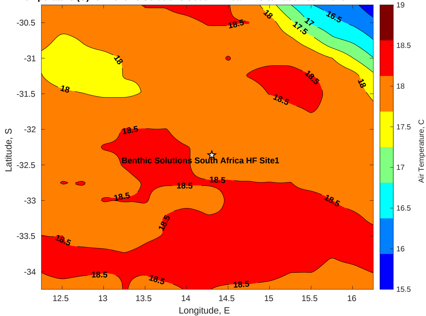
Air Temperature (C) for Benthic Solutions South Africa HF Site1 at 07-Jun-2025
