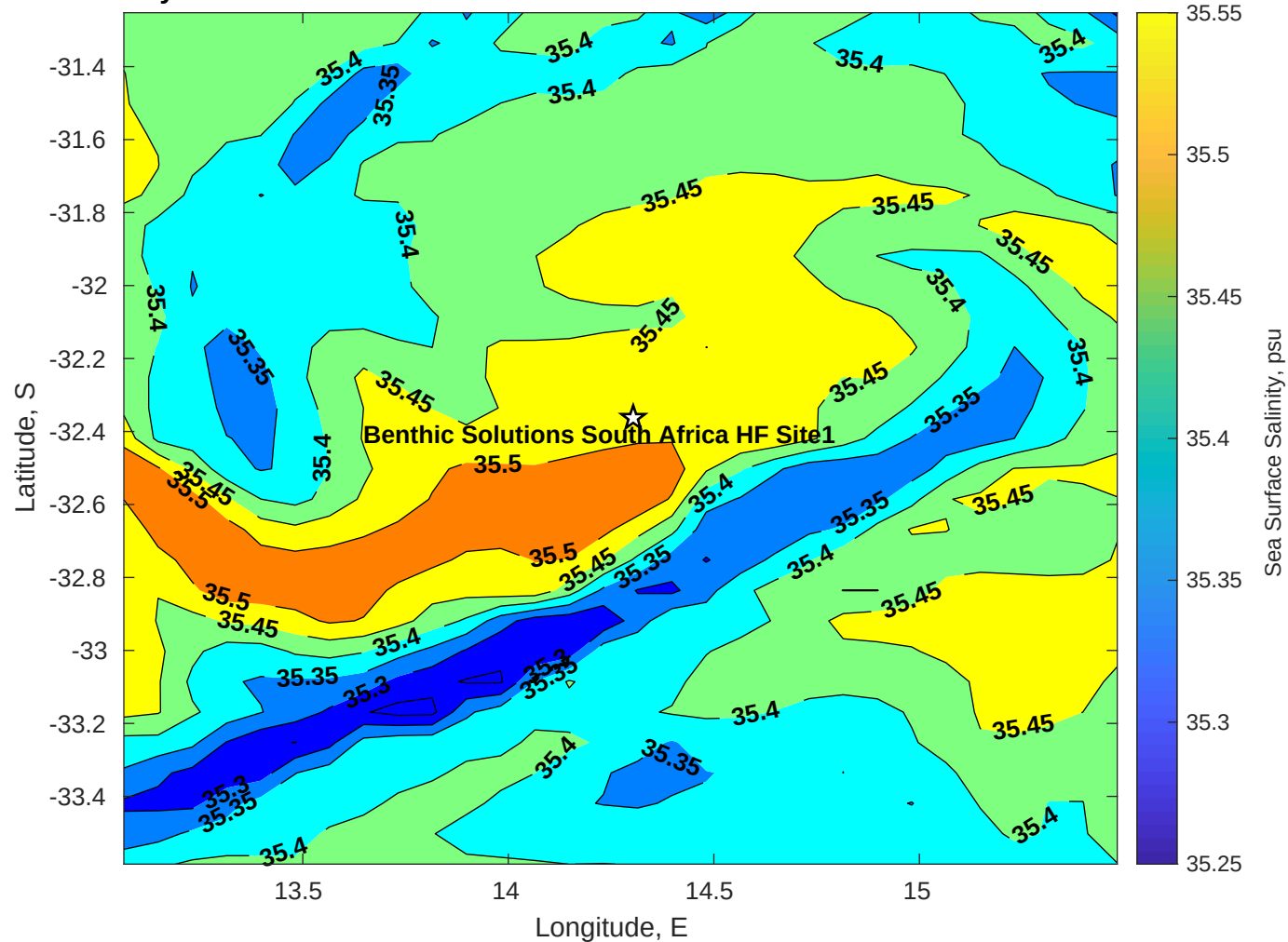
Surface Salinity for Benthic Solutions South Africa HF Site1 at 06-Jun-2025 00:00:00
