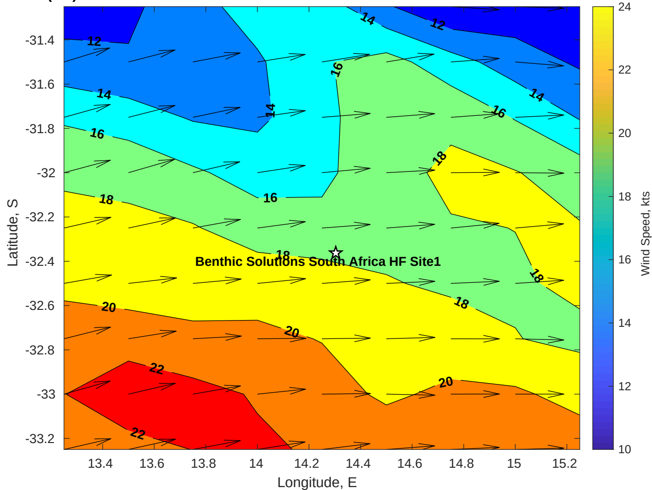
Winds (kts) for Benthic Solutions South Africa HF Site1 at 07-Jun-2025 09:00:00
