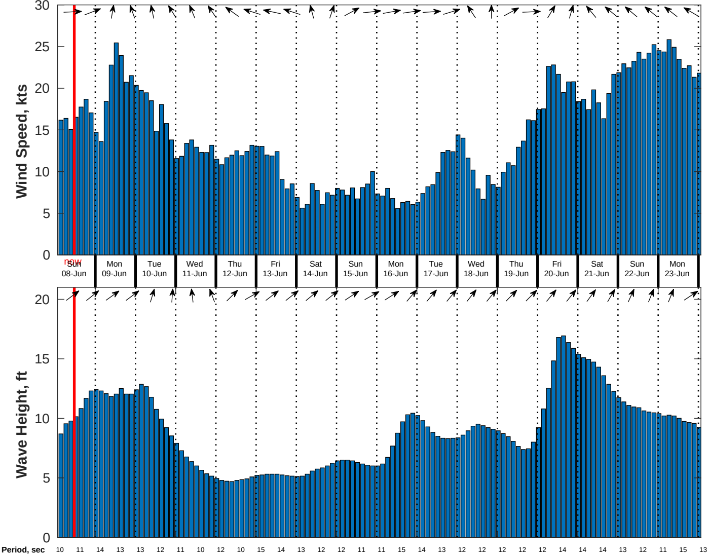
Wind & Wave Forecast for Benthic Solutions South Africa HF Site1 from 07-Jun-2025 02:00:00 to 23-Jun-2025 02:00:00
