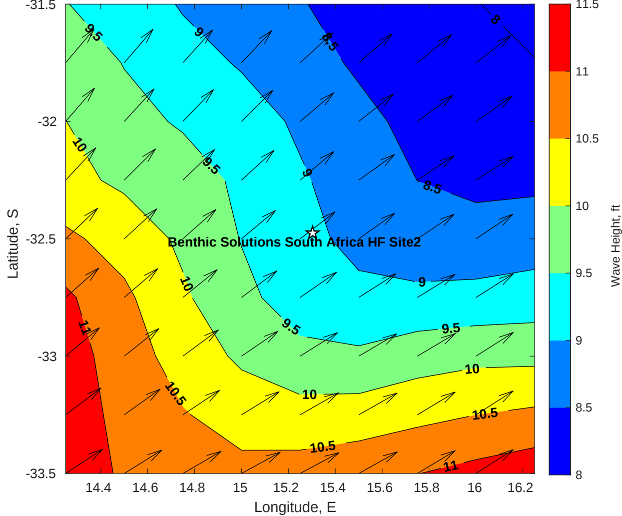
Wave Height (ft) for Benthic Solutions South Africa HF Site2 at 07-Jun-2025 09:00:00
