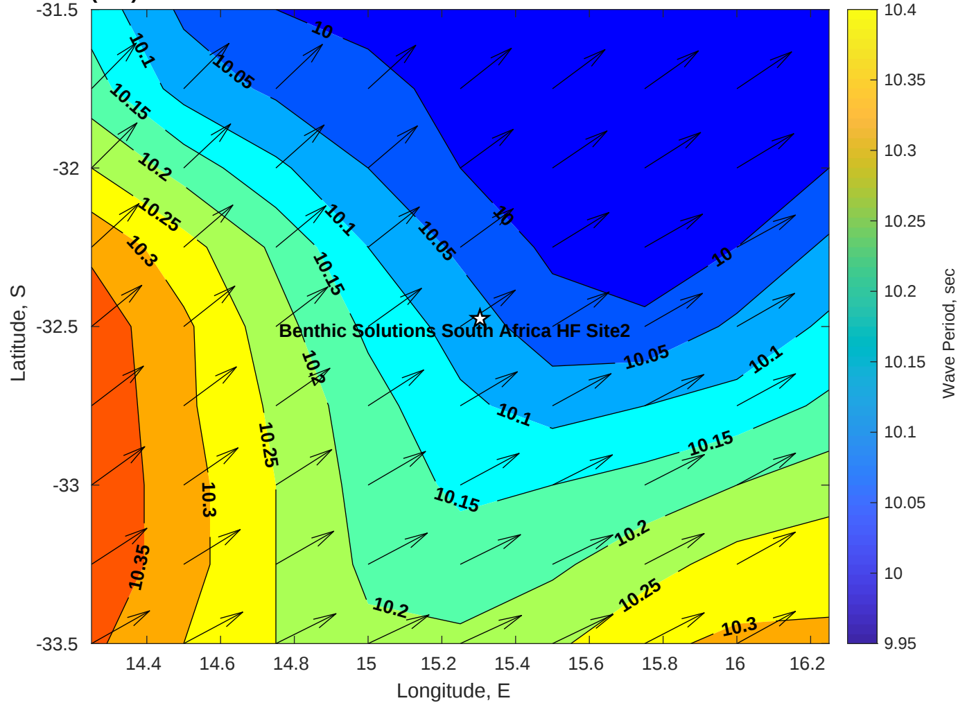
Wave Period (sec) for Benthic Solutions South Africa HF Site2 at 07-Jun-2025 09:00:00
