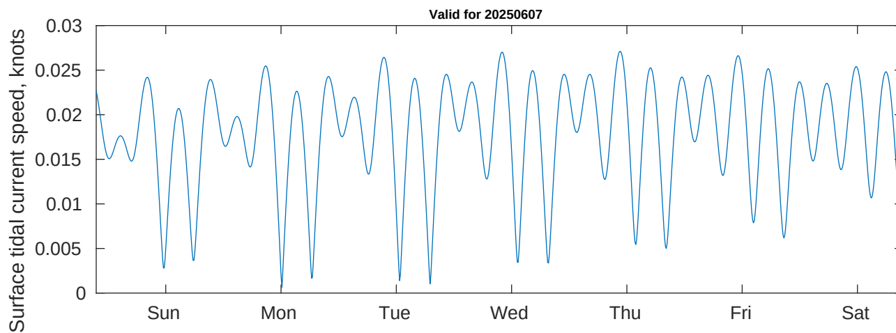
Tidal Currents and Heights for Benthic Solutions South Africa HF Site2 at 20250607
