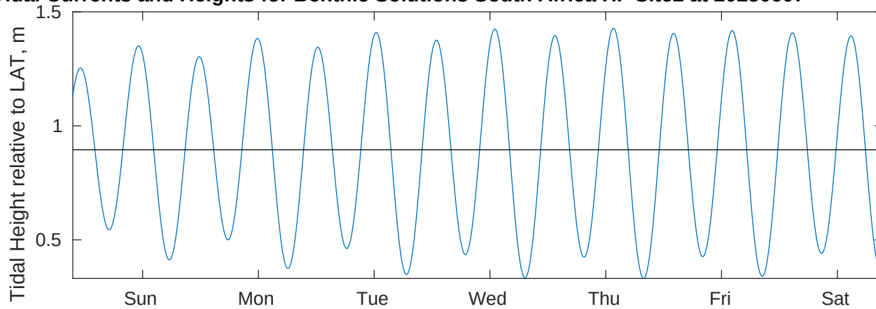
Tidal Currents and Heights for Benthic Solutions South Africa HF Site2 at 20250607
