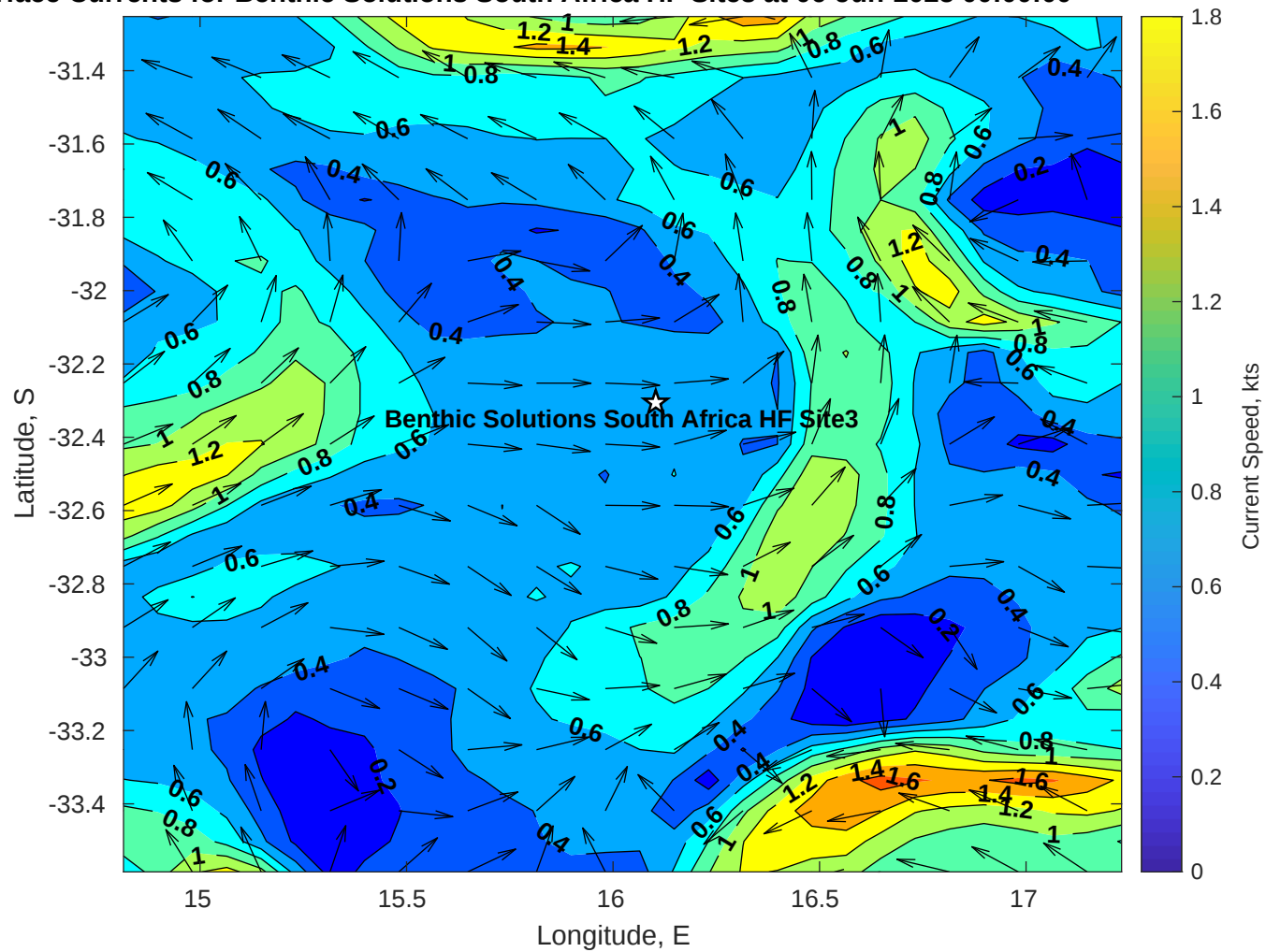
Surface Currents for Benthic Solutions South Africa HF Site3 at 06-Jun-2025 00:00:00
