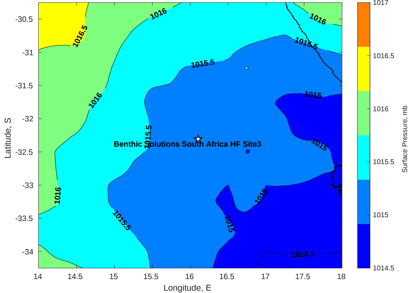
Surface Pressure (mb) for Benthic Solutions South Africa HF Site3 at 08-Jun-2025 00:00:00
