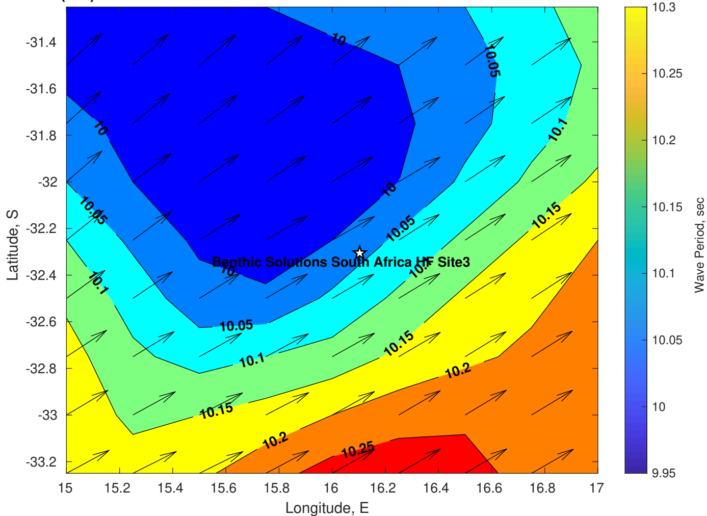
Wave Period (sec) for Benthic Solutions South Africa HF Site3 at 07-Jun-2025 09:00:00
