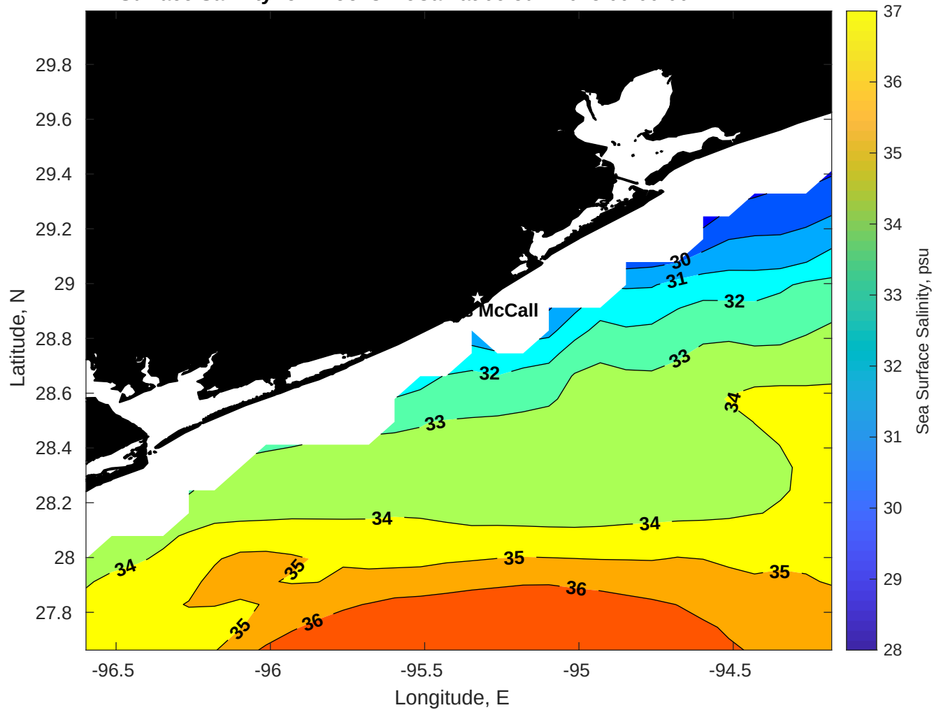
Surface Salinity for Brooks McCall at 06-Jun-2025 00:00:00
