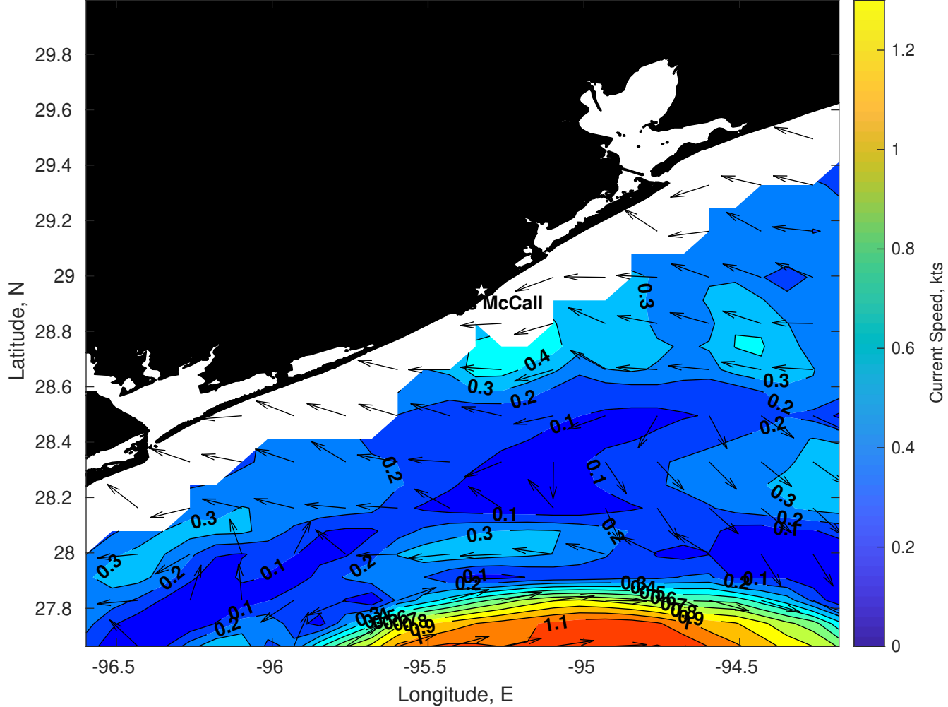
Surface Currents for Brooks McCall at 06-Jun-2025 00:00:00
