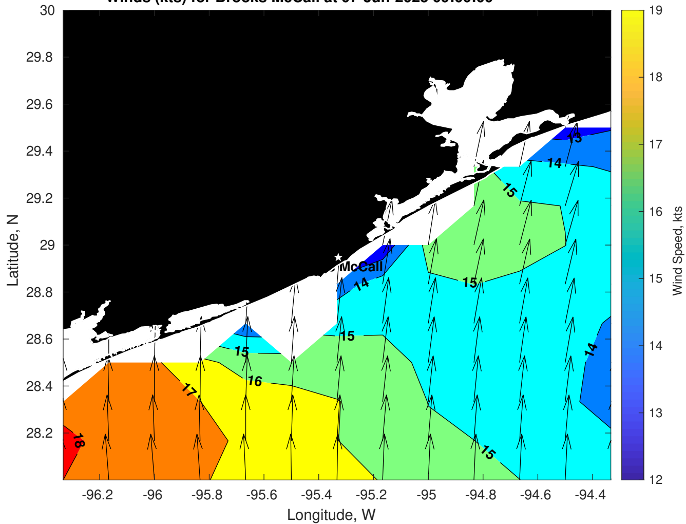
Winds (kts) for Brooks McCall at 07-Jun-2025 09:00:00
