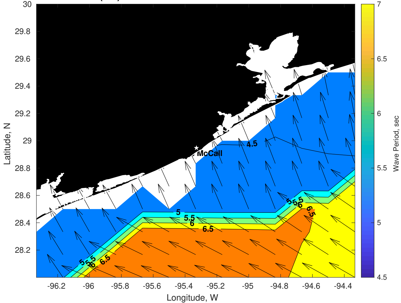
Wave Period (sec) for Brooks McCall at 07-Jun-2025 09:00:00
