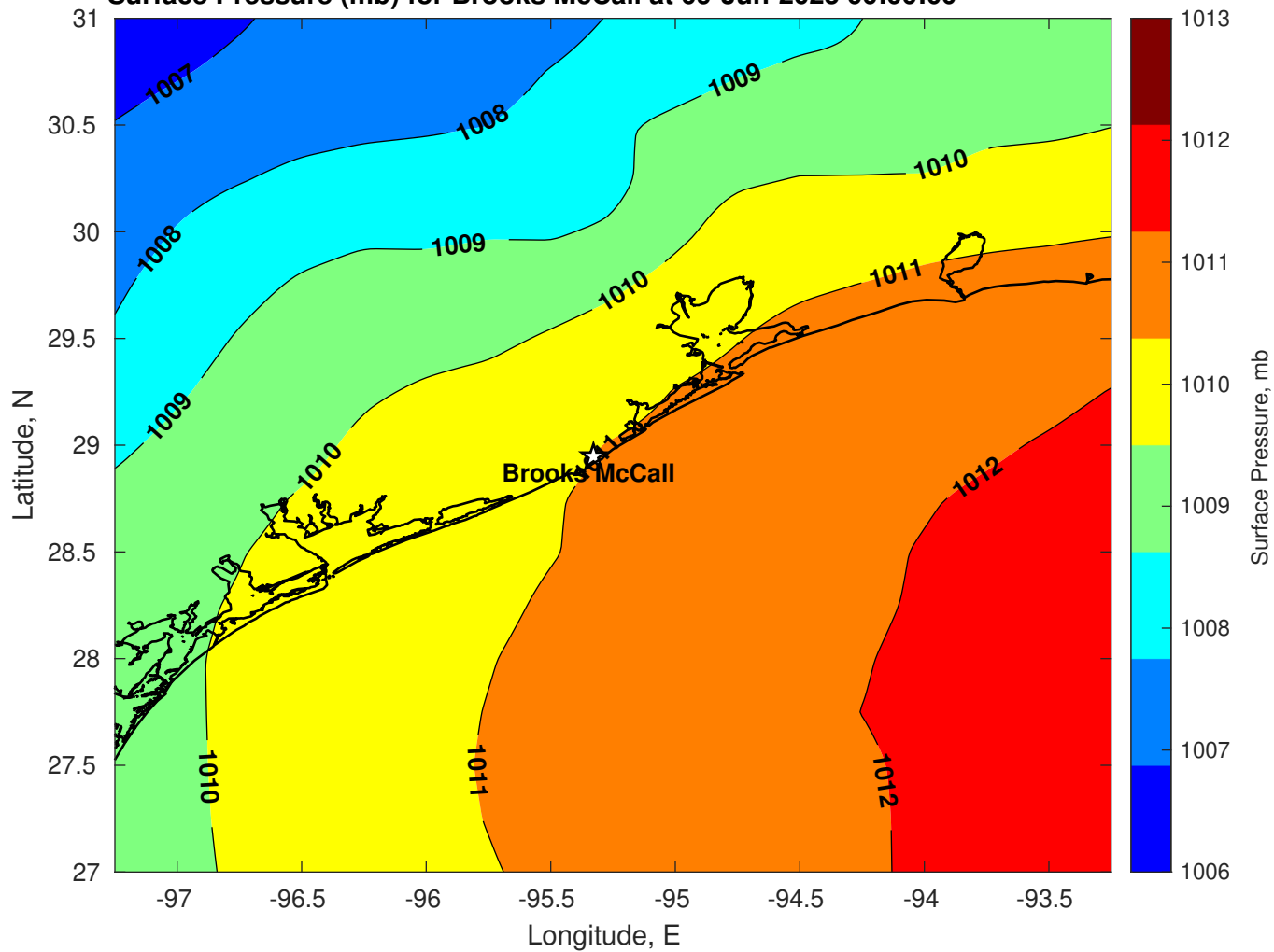
Surface Pressure (mb) for Brooks McCall at 09-Jun-2025 00:00:00
