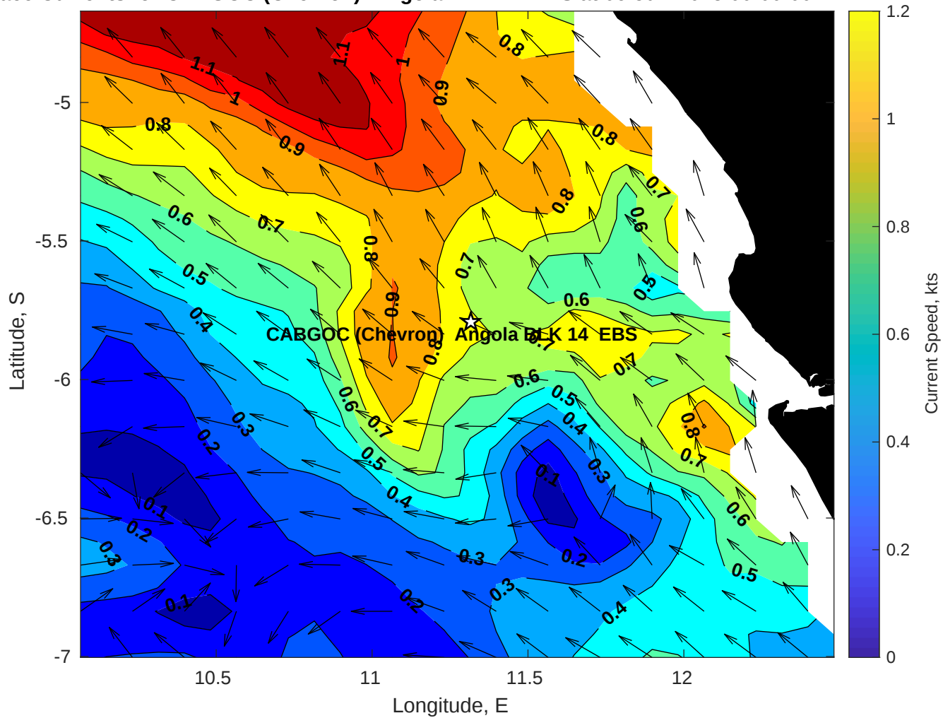
Surface Currents for CABGOC (Chevron) Angola BLK 14 EBS at 06-Jun-2025 00:00:00
