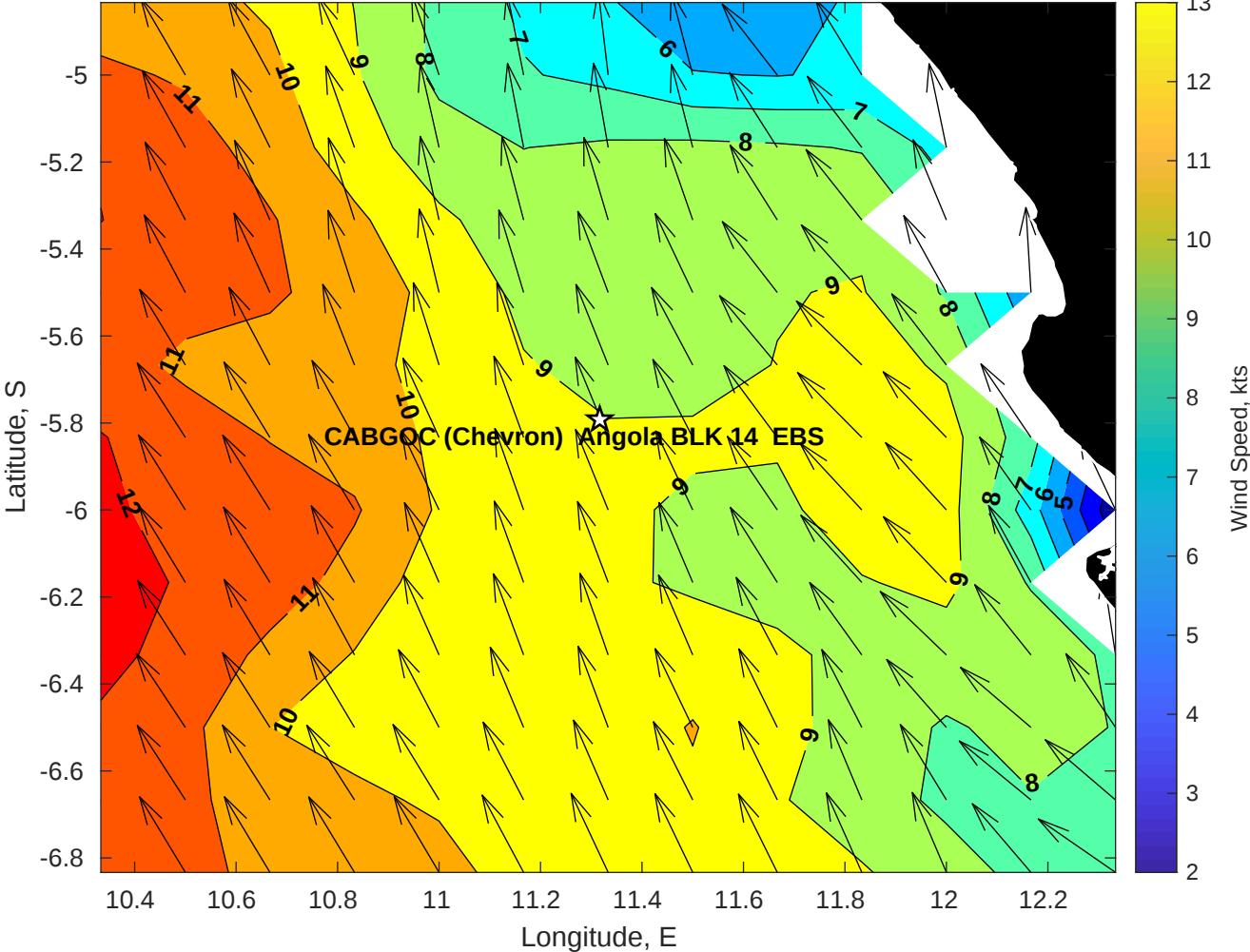
Winds (kts) for CABGOC (Chevron) Angola BLK 14 EBS at 07-Jun-2025 09:00:00
