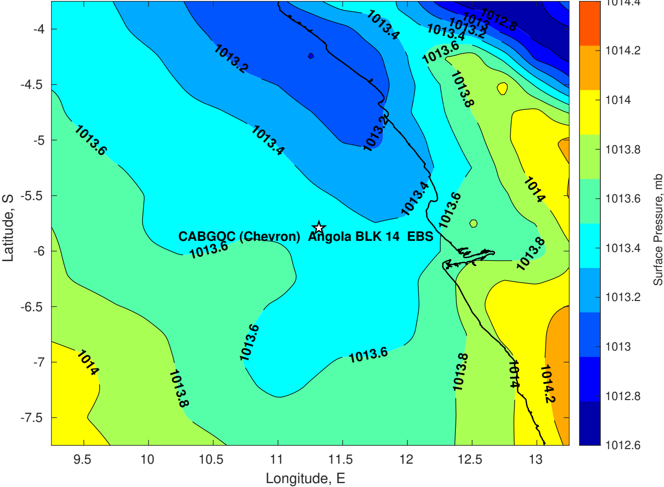
Surface Pressure (mb) for CABGOC (Chevron) Angola BLK 14 EBS at 09-Jun-2025 00:00:00
