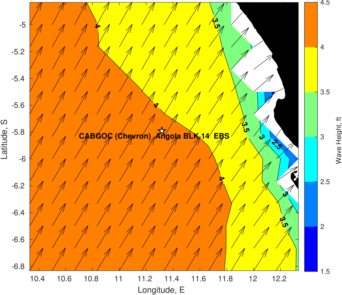
Wave Height (ft) for CABGOC (Chevron) Angola BLK 14 EBS at 07-Jun-2025 09:00:00
