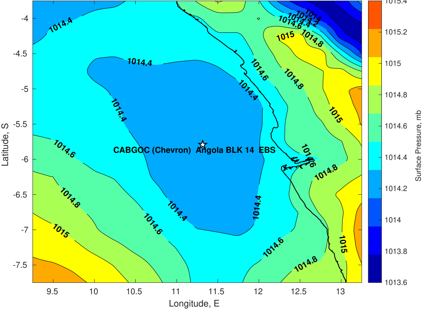
Surface Pressure (mb) for CABGOC (Chevron) Angola BLK 14 EBS at 07-Jun-2025 00:00:00
