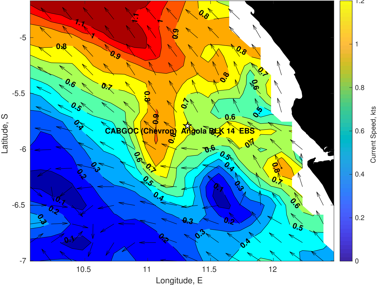
Surface Currents for CABGOC (Chevron) Angola BLK 14 EBS at 06-Jun-2025 00:00:00
