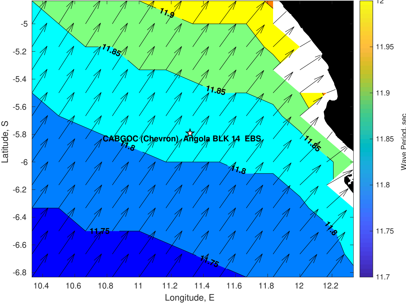
Wave Period (sec) for CABGOC (Chevron) Angola BLK 14 EBS at 07-Jun-2025 09:00:00
