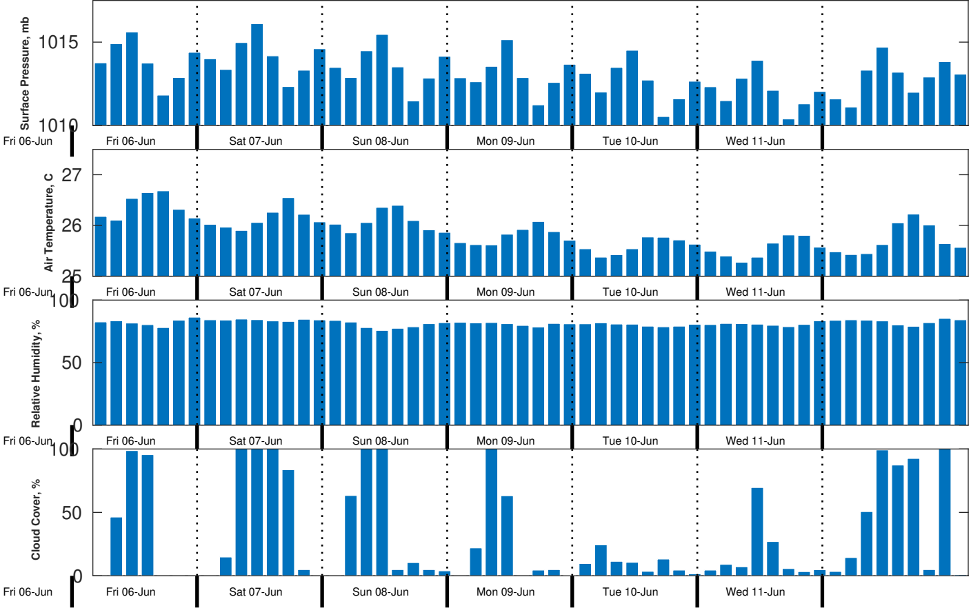
Met Forecast for CABGOC (Chevron) Angola BLK 14 EBS from 07-Jun-2025 00:00:00 to 14-Jun-2025 00:00:00
