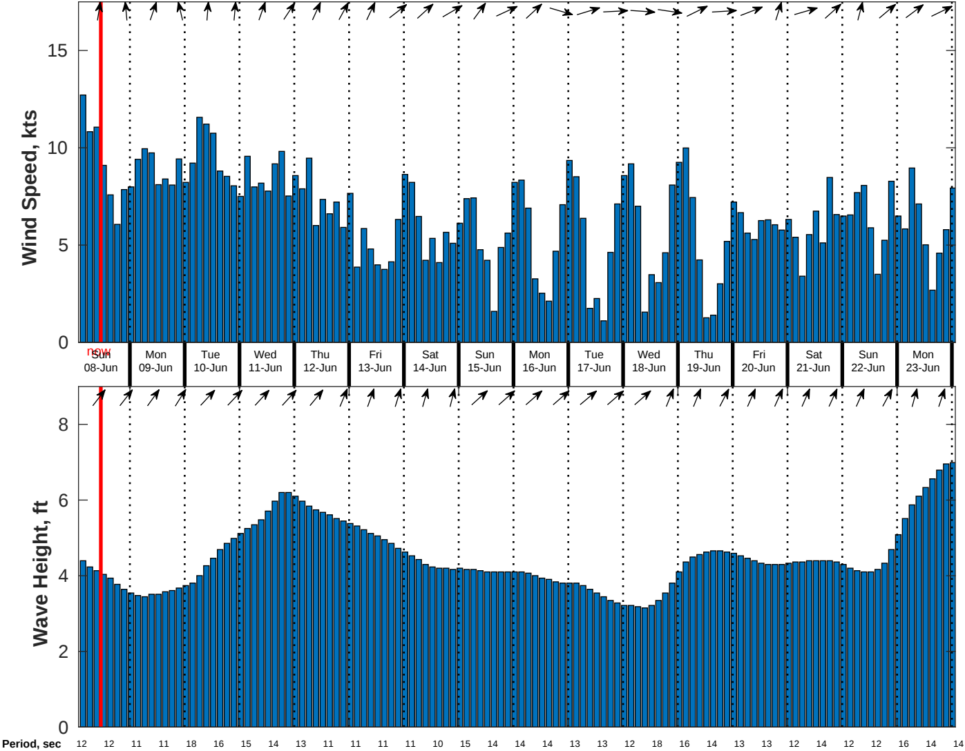
Wind & Wave Forecast for CABGOC (Chevron) Angola BLK 14 EBS from 07-Jun-2025 02:00:00 to 23-Jun-2025 02:00:00
