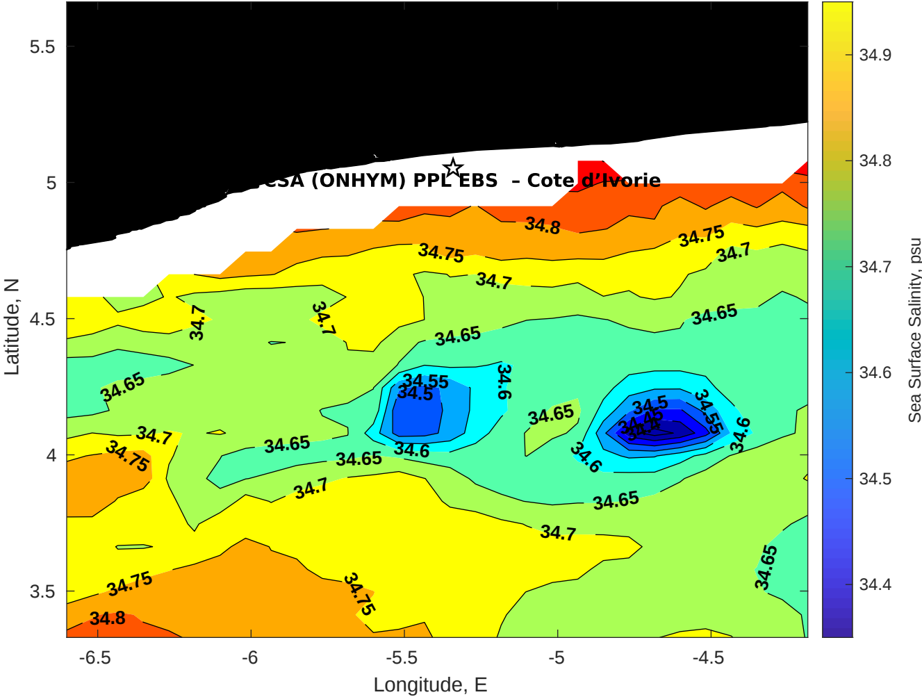
Surface Salinity for CSA (ONHYM) PPL EBS - Cote d'Ivoire at 06-Jun-2025 00:00:00
