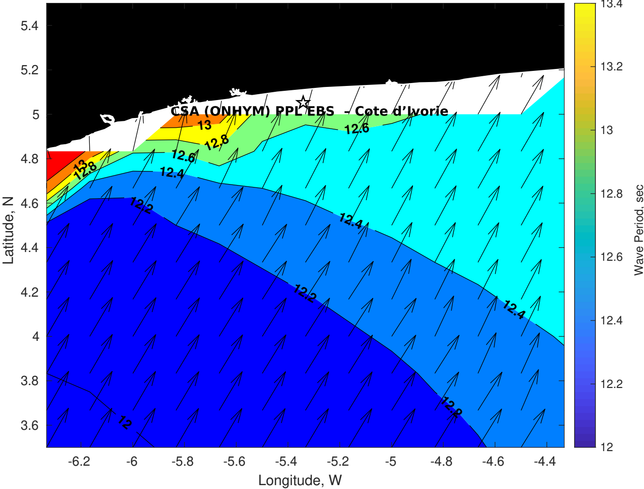
Wave Period (sec) for CSA (ONHYM) PPL EBS - Cote d'Ivoire at 07-Jun-2025 09:00:00
