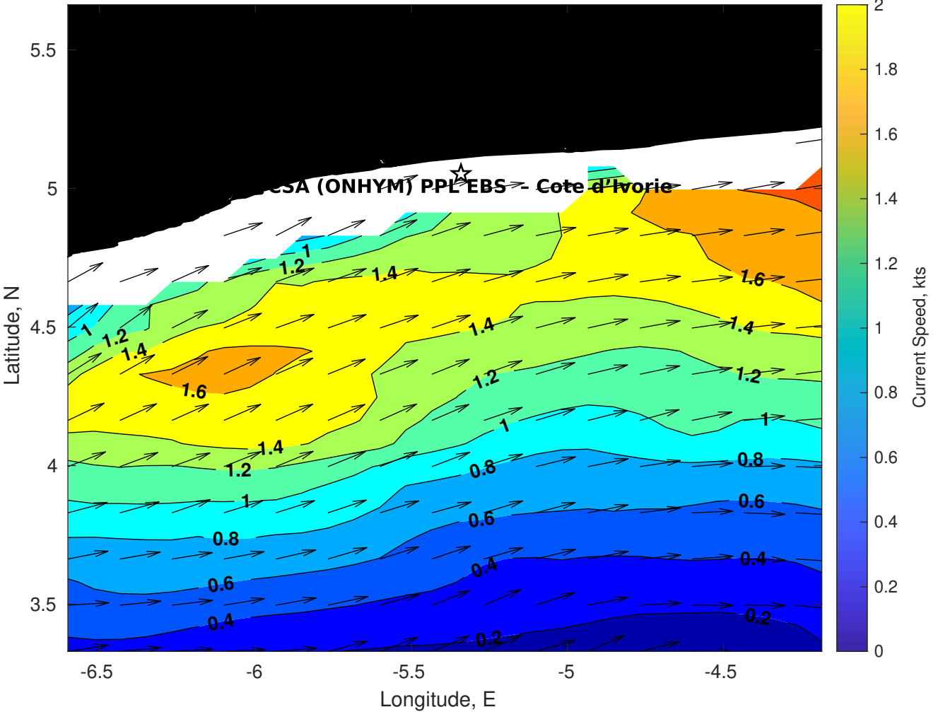
Surface Currents for CSA (ONHYM) PPL EBS - Cote d'Ivoire at 06-Jun-2025 00:00:00
