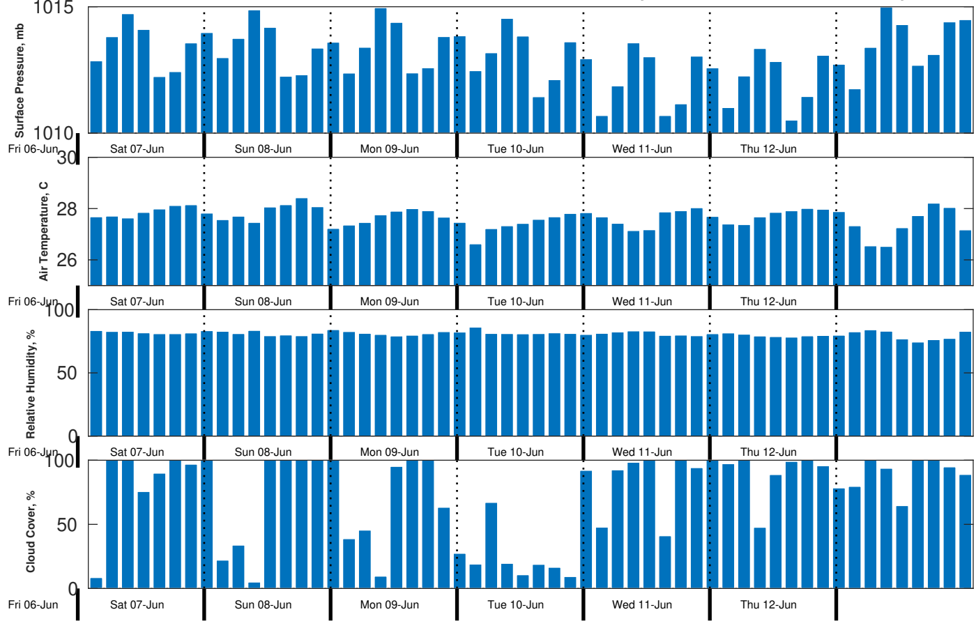
Met Forecast for CSA (ONHYM) PPL EBS - Cote d'Ivoire from 07-Jun-2025 00:00:00 to 14-Jun-2025 00:00:00
