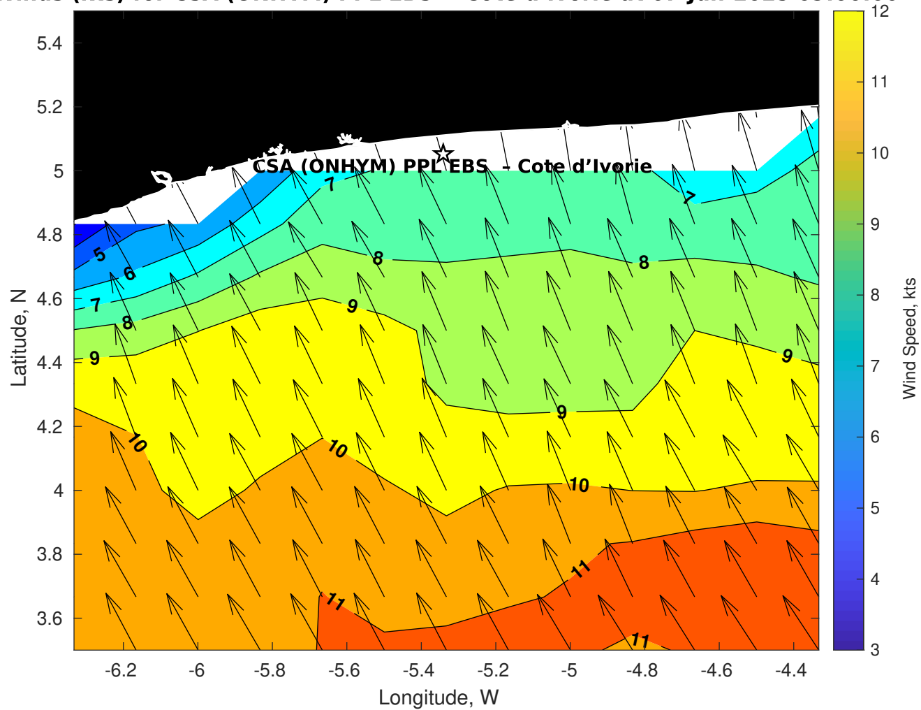
Winds (kts) for CSA (ONHYM) PPL EBS - Cote d'Ivoire at 07-Jun-2025 09:00:00
