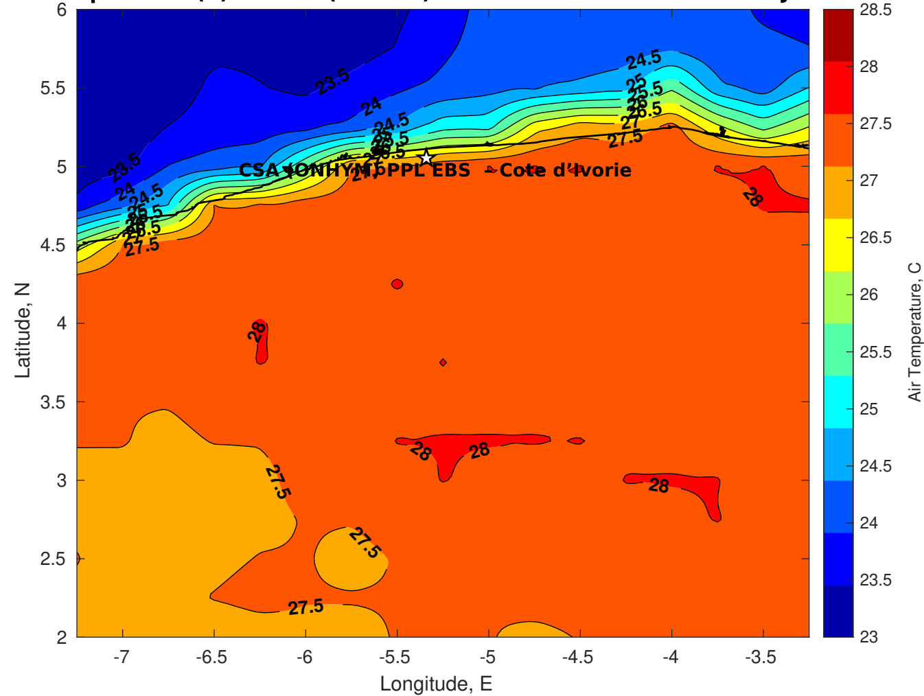
Air Temperature (C) for CSA (ONHYM) PPL EBS - Cote d'Ivoire at 07-Jun-2025
