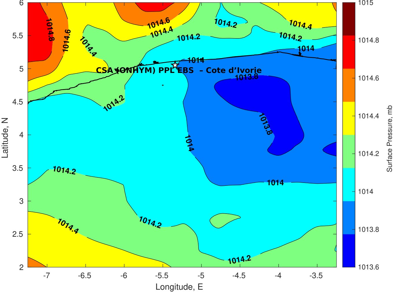
Surface Pressure (mb) for CSA (ONHYM) PPL EBS - Cote d'Ivoire at 08-Jun-2025 00:00:00
