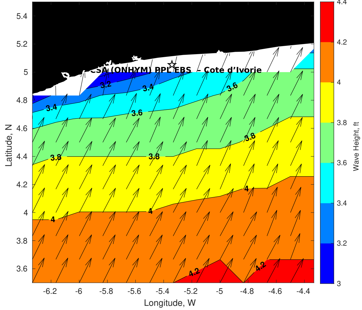
Wave Height (ft) for CSA (ONHYM) PPL EBS - Cote d'Ivoire at 07-Jun-2025 09:00:00
