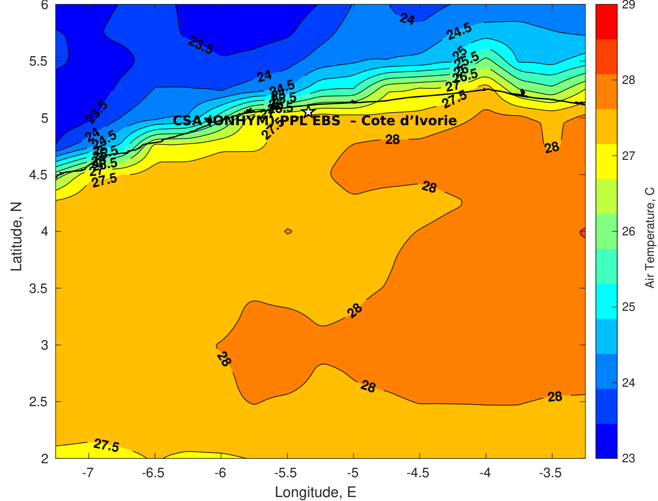
Air Temperature (C) for CSA (ONHYM) PPL EBS - Cote d'Ivoire at 07-Jun-2025
