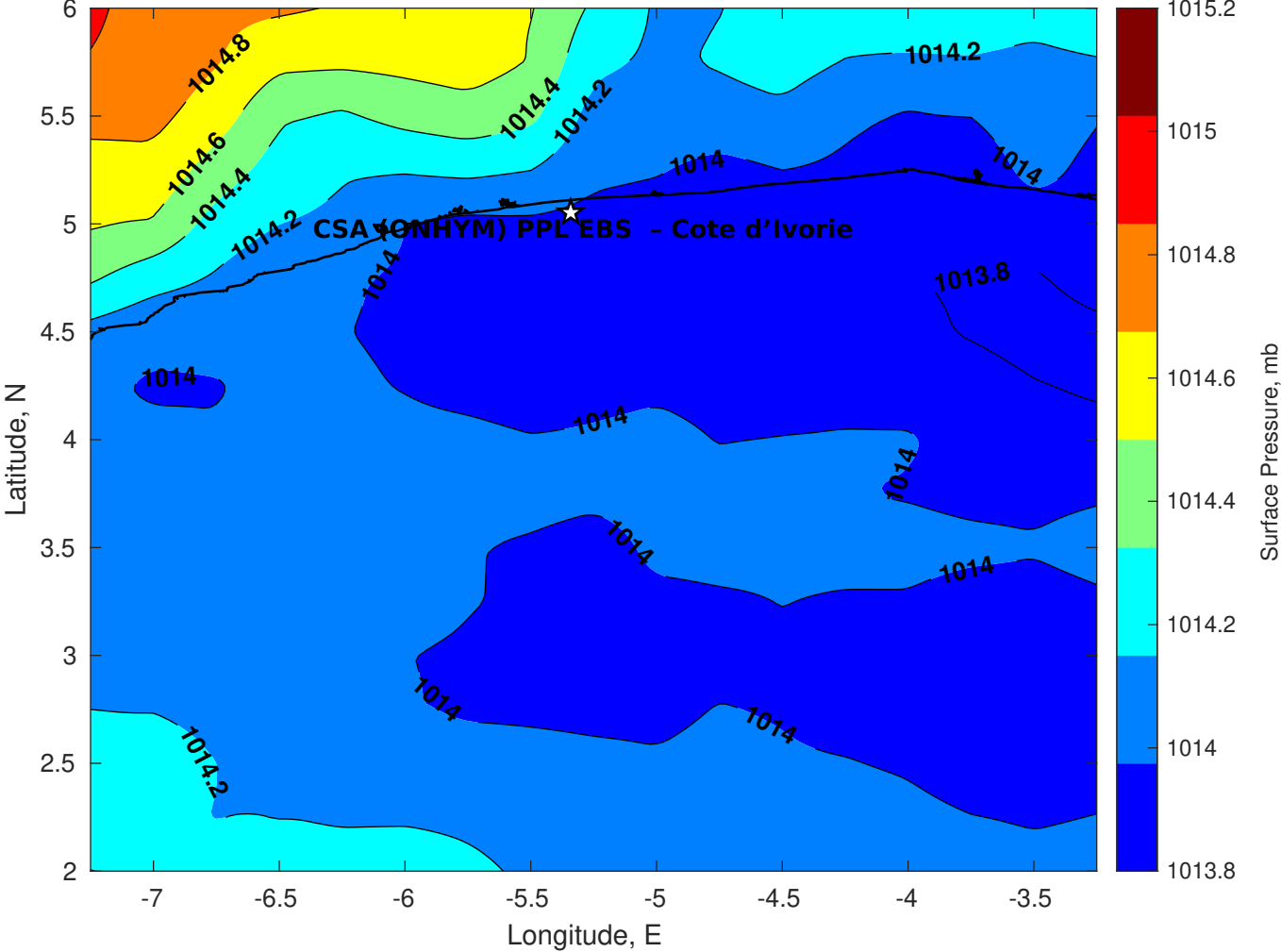
Surface Pressure (mb) for CSA (ONHYM) PPL EBS - Cote d'Ivoire at 07-Jun-2025 00:00:00
