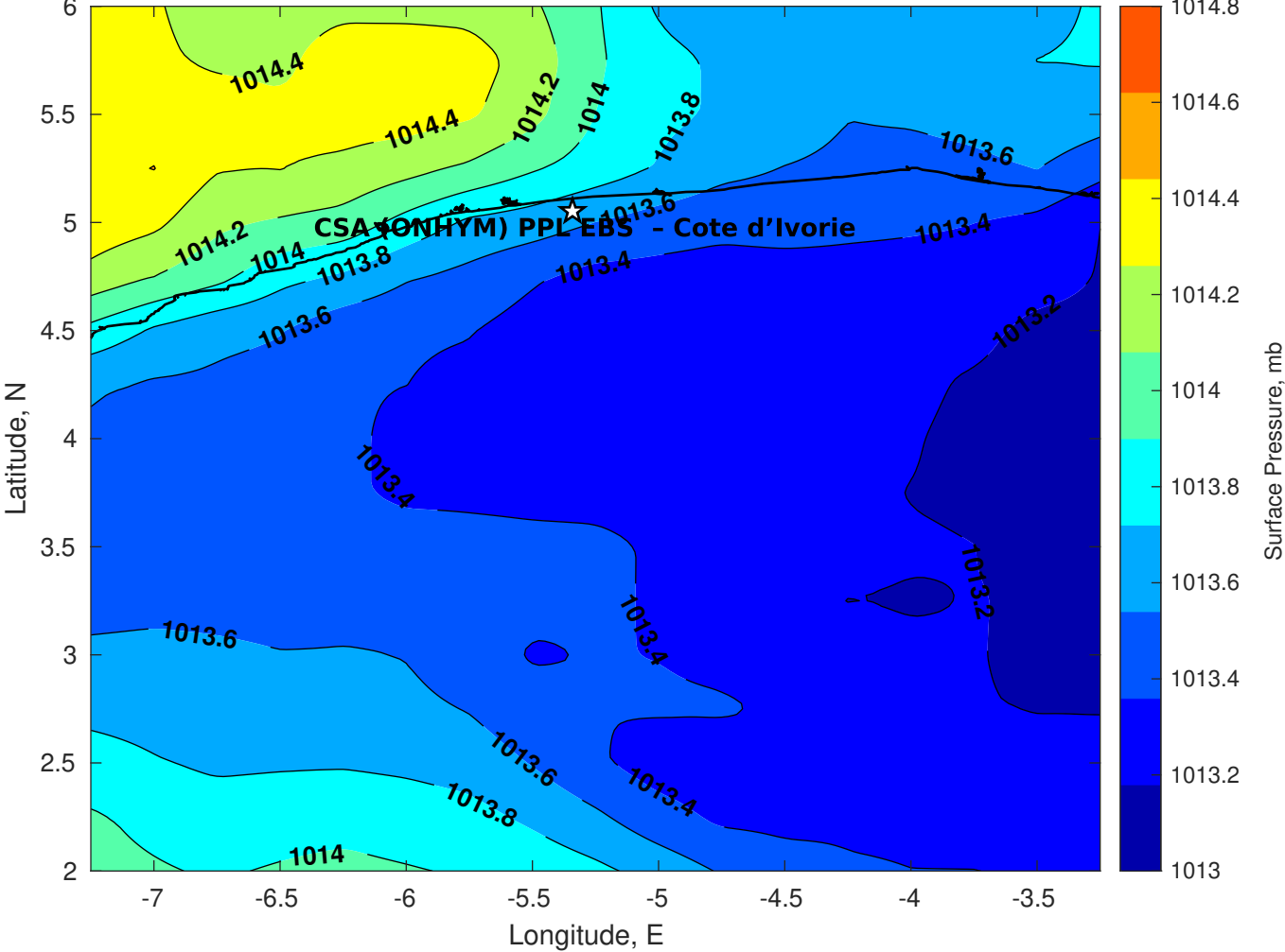
Surface Pressure (mb) for CSA (ONHYM) PPL EBS - Cote d'Ivoire at 09-Jun-2025 00:00:00
