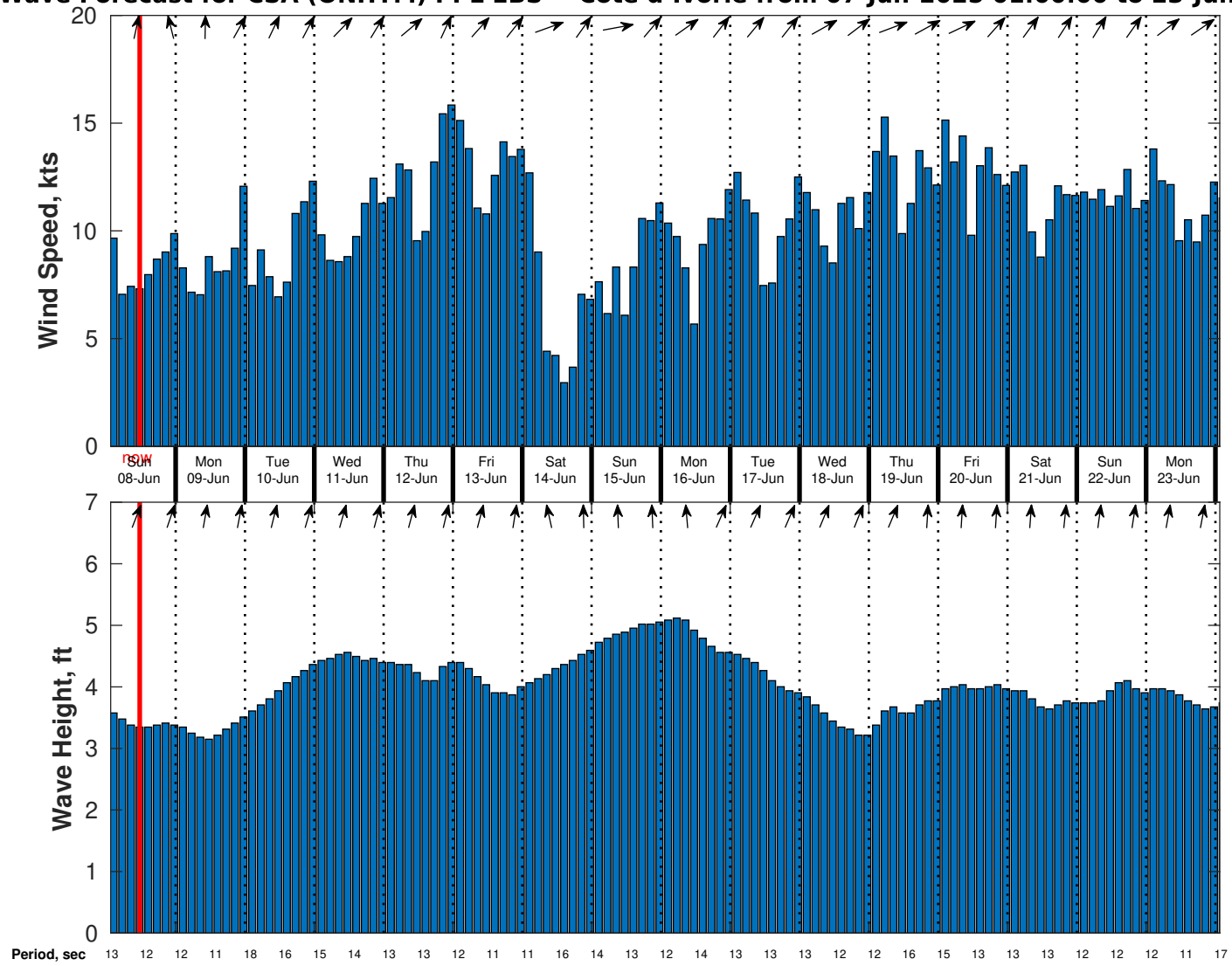
Wind & Wave Forecast for CSA (ONHYM) PPL EBS - Cote d'Ivoire from 07-Jun-2025 01:00:00 to 23-Jun-2025 01:00:00
