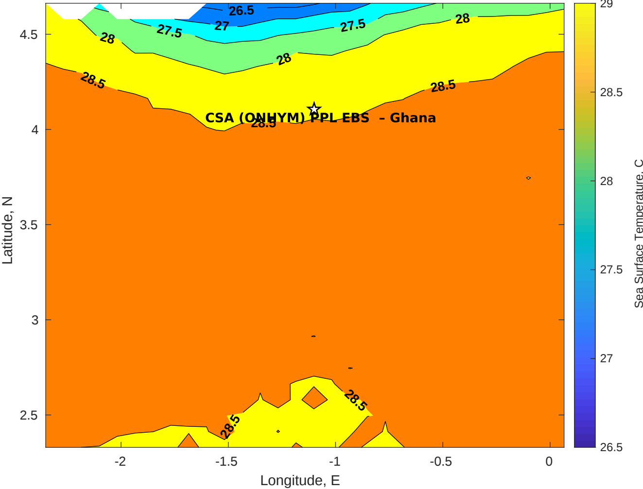
SST for CSA (ONHYM) PPL EBS - Ghana at 06-Jun-2025 00:00:00
