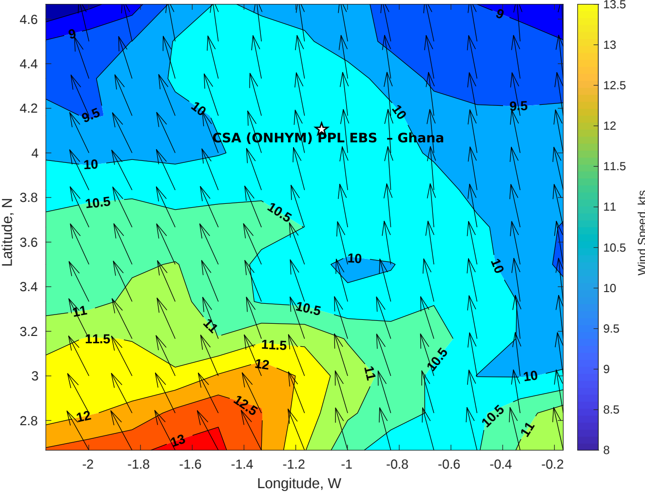
Winds (kts) for CSA (ONHYM) PPL EBS - Ghana at 07-Jun-2025 09:00:00
