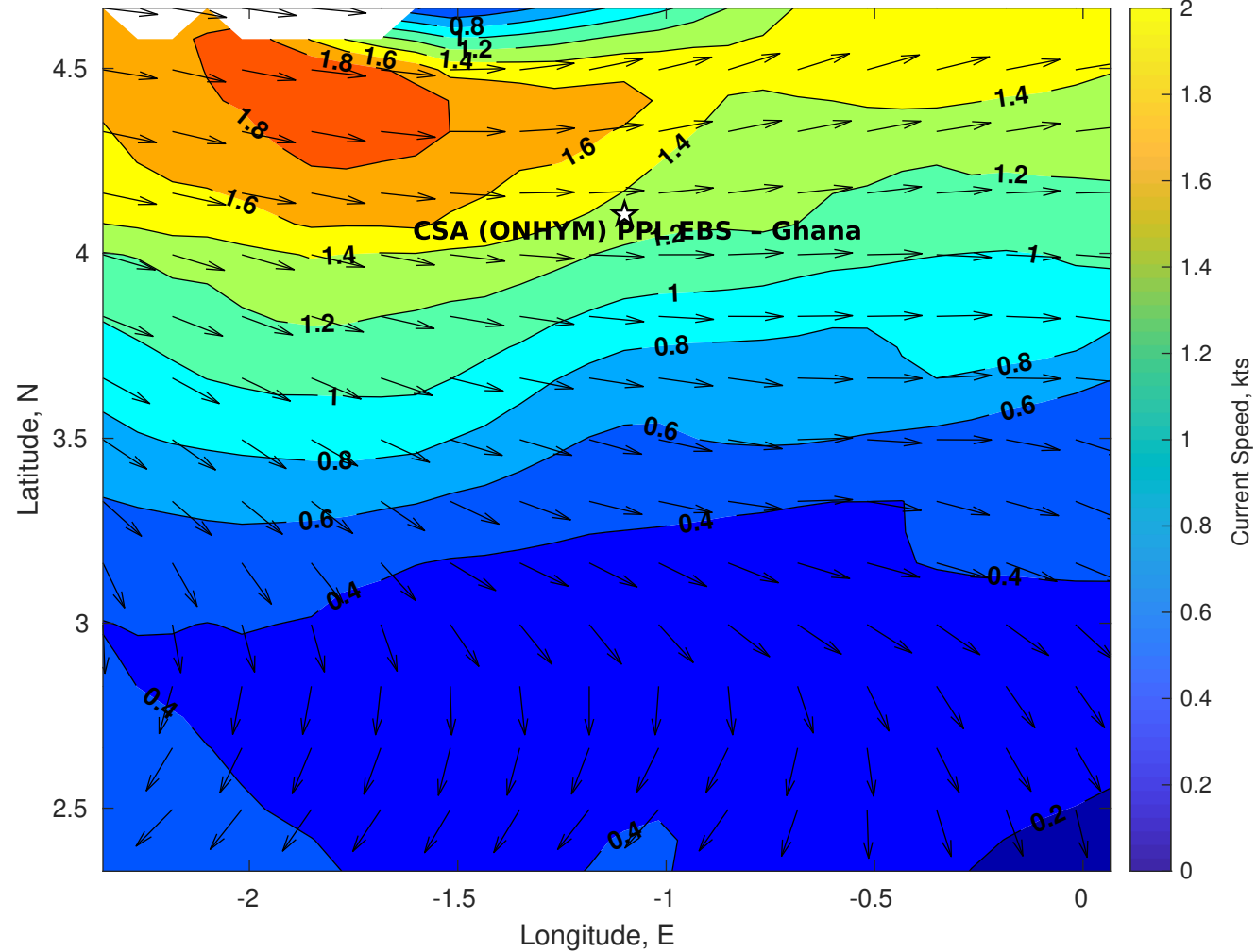
Surface Currents for CSA (ONHYM) PPL EBS - Ghana at 06-Jun-2025 00:00:00
