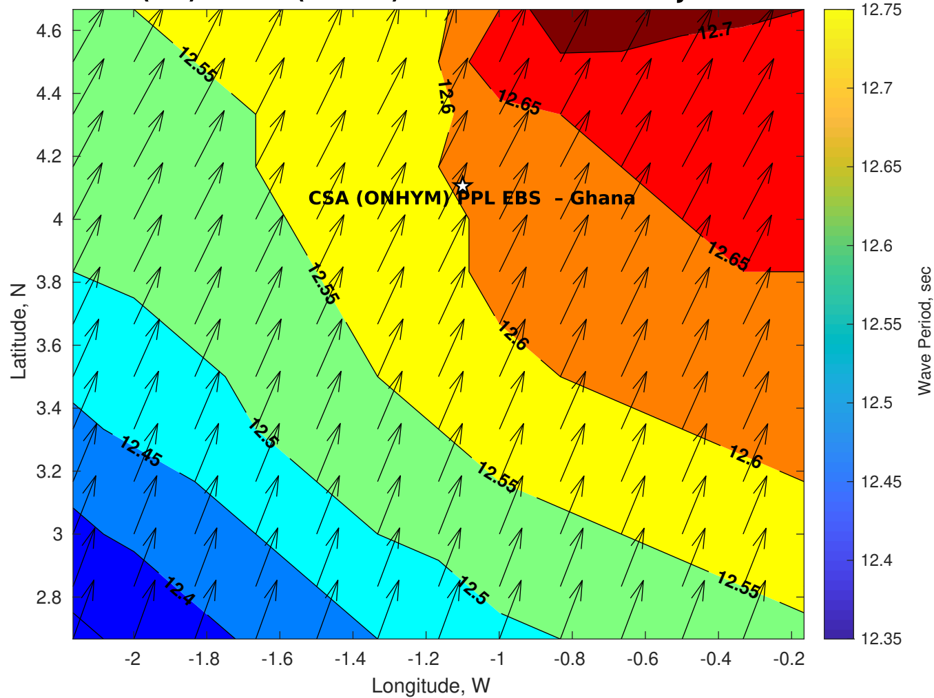
Wave Period (sec) for CSA (ONHYM) PPL EBS - Ghana at 07-Jun-2025 09:00:00
