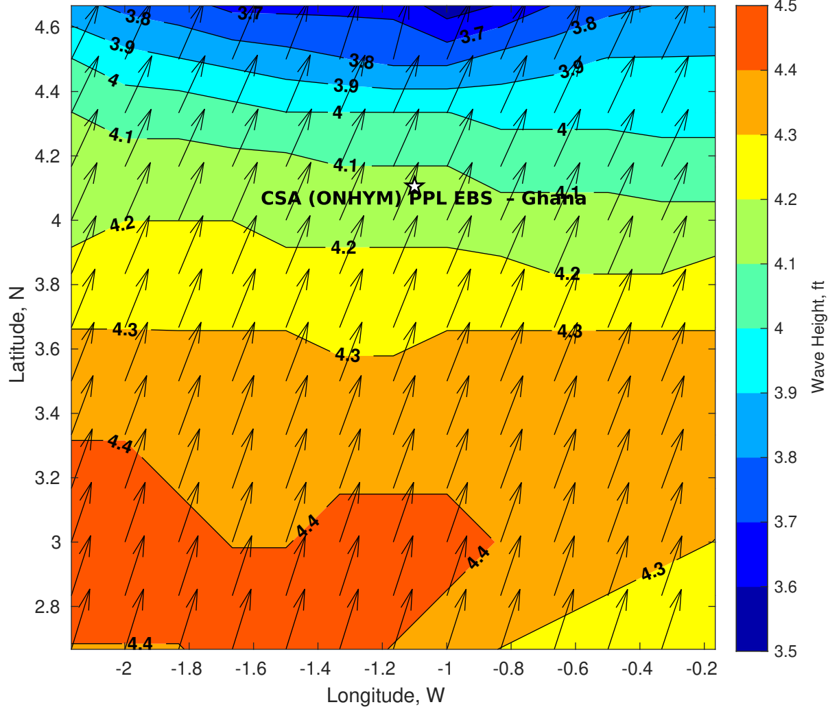
Wave Height (ft) for CSA (ONHYM) PPL EBS - Ghana at 07-Jun-2025 09:00:00
