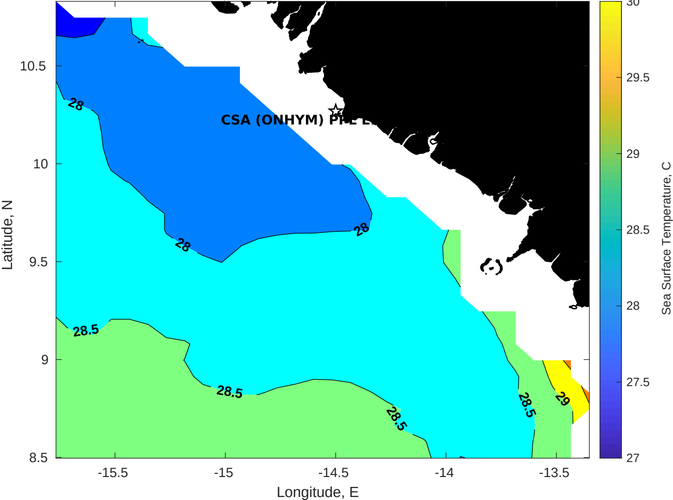
SST for CSA (ONHYM) PPL EBS - Guinea at 06-Jun-2025 00:00:00
