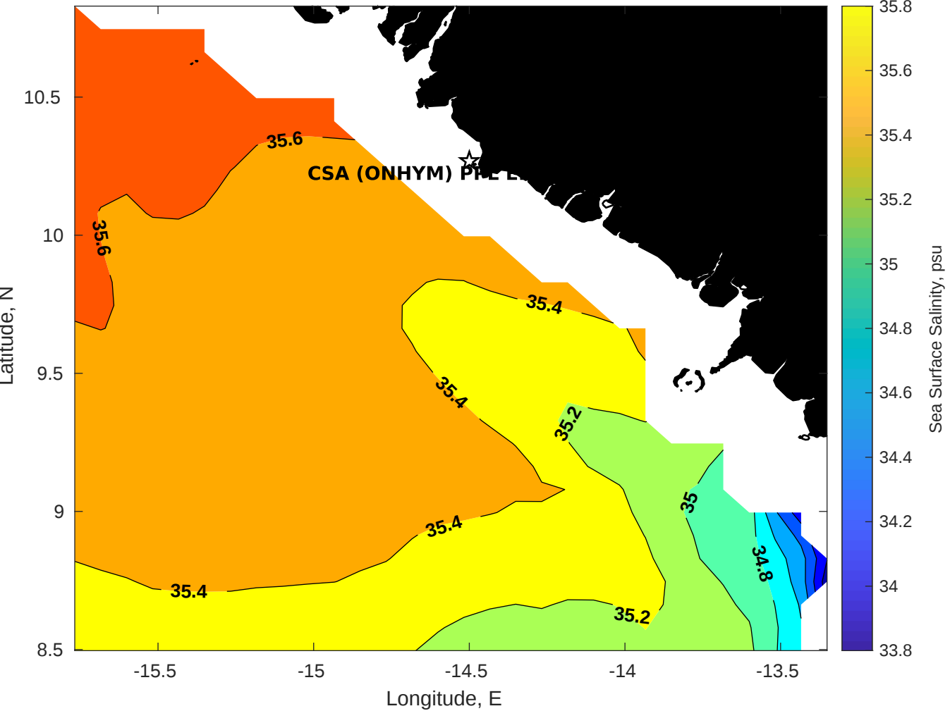
Surface Salinity for CSA (ONHYM) PPL EBS - Guinea at 06-Jun-2025 00:00:00
